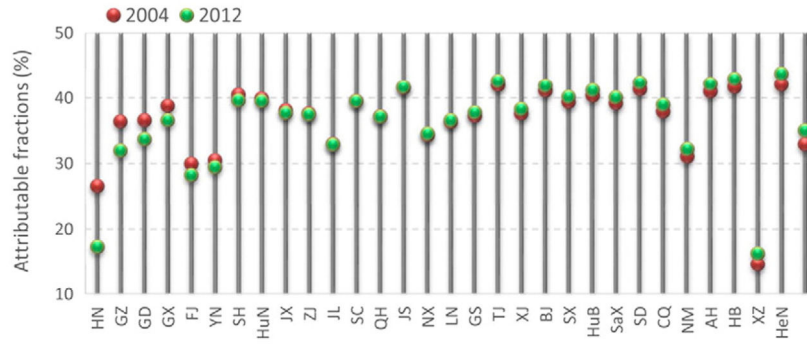
Fig. 4. Averaged attributable fractions of total deaths for 31 provinces of China. Total deaths here are the sum of deaths caused by lung cancer, IHD and stroke.
