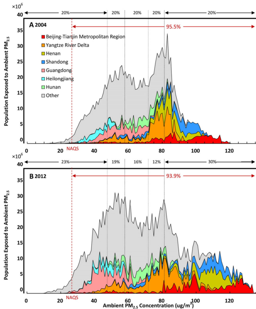
Fig. 1. National and provincial distribution of population as a function of ambient PM 2.5 concentration in 2004 (A) and 2012 (B). Red dash vertical lines (in both plots) indicate the annual concentration limits in China's National Air Quality Standard for GradeII. Grey dash vertical lines (in both plots) demarcate boundaries of population quintiles that apportion the PM 2.5 concentration distribution into 5 bins with equal number of exposed population in 2004.
