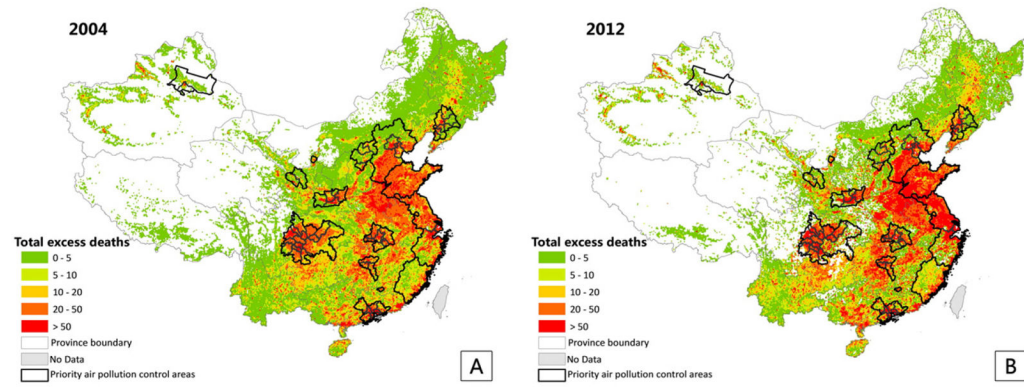
Fig. 3. Spatial distributions of total excess deaths attributable to PM 2.5 exposure in 2004 (A) and 2012 (B) (cases per 100 km 2 ). Total deaths here are the sum of deaths caused by lung cancer, IHD and stroke. Black lines show the boundary of priority areas of national joint air pollution prevention and control.
