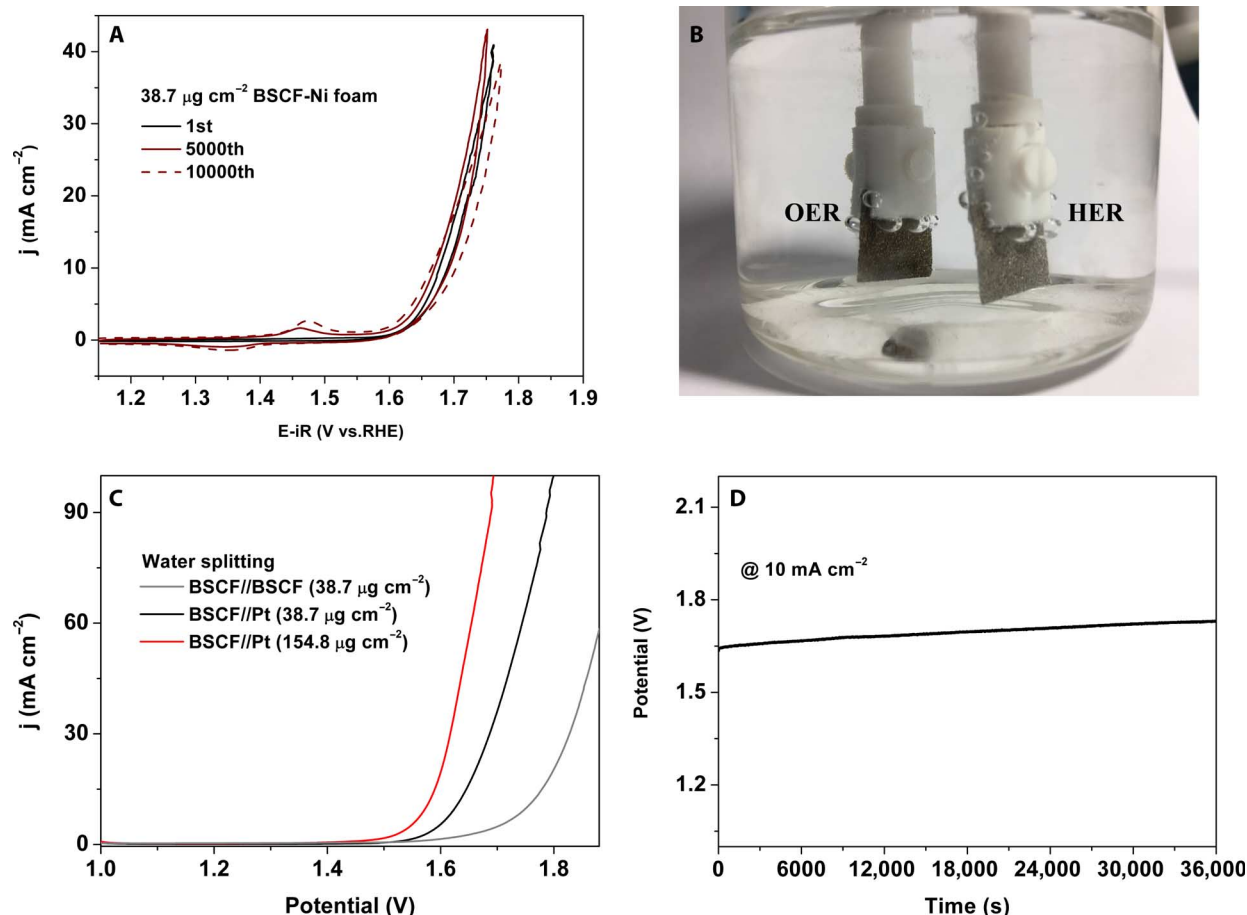
Fig. 4. Electrochemical behaviors of amorphous BSCF nanofilms on Ni foam substrates. (A) Current-potential profile at the 1st, 5000th, and 10,000th cycles for the 38.7 μg cm -2 BSCF-Ni foam heterostructure electrode in a 0.1 M KOH solution. (B) Two-electrode electrolyzer setup consisting of 38.7 μg cm -2 BSCF-Ni foam anode and 38.7 μg cm -2 Pt-Ni foam cathode in a 1.0 M KOH solution. (C) Typical current-potential profiles from the two-electrode electrolyzer during water splitting. (D) Time-dependent potential response during 10-hour chronoamperometric water-splitting reaction using the two-electrode electrolyzer (38.7 μg cm -2 BSCF-Ni foam anode and 38.7 μg cm -2 Pt-Ni foam cathode) at a constant current density of 10 mA cm -2 .
