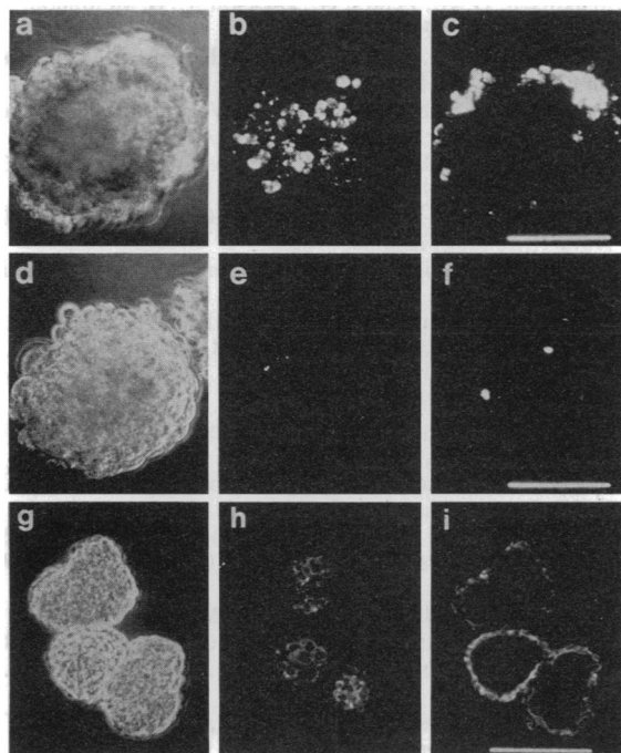
FIG. 5. Fluorescence assay for \beta -gal activity in vivo and immunofluorescent detection of SPARC antigen. Embryoid bodies prepared from 62-8K (a, b, c) and CC1.2 (d, e, f) cells were incubated with FDG (substrate) and fluorescein (product) was detected by using confocal laser scanning microscopy. 62-8K embryoid bodies (g, h, i) were fixed and incubated sequentially with rabbit anti-SPARC serum and donkey anti-rabbit IgG coupled with Texas red. Phase-contrast images are shown on the left (a, d, g). Two fluorescence images in different focal planes are shown for each embryoid body: a section near the surface (b, e, h) and a section 22.5 \mu m deeper than the first (c, f, i). The section thickness is approximately 7 \mu m. The scale bars indicate 100 \mu m.
