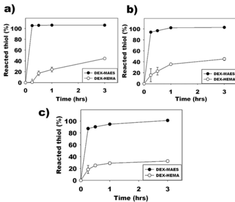
Figure 3. Quantification of reacted thiol after reacting (a) 5 mg, (b) 10 mg and (c) 20 mg GRGDSPC to 1g DEX-MAES and DEX-HEMA macromers.
