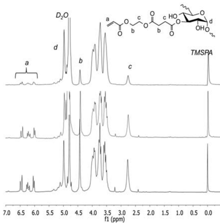
Figure 2. Proton NMR spectra of DEX-MAES with various degrees of MAES modification.
