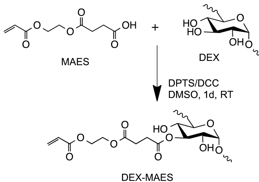
Figure 1. Schematic illustration of DEX-MAES synthesis.
