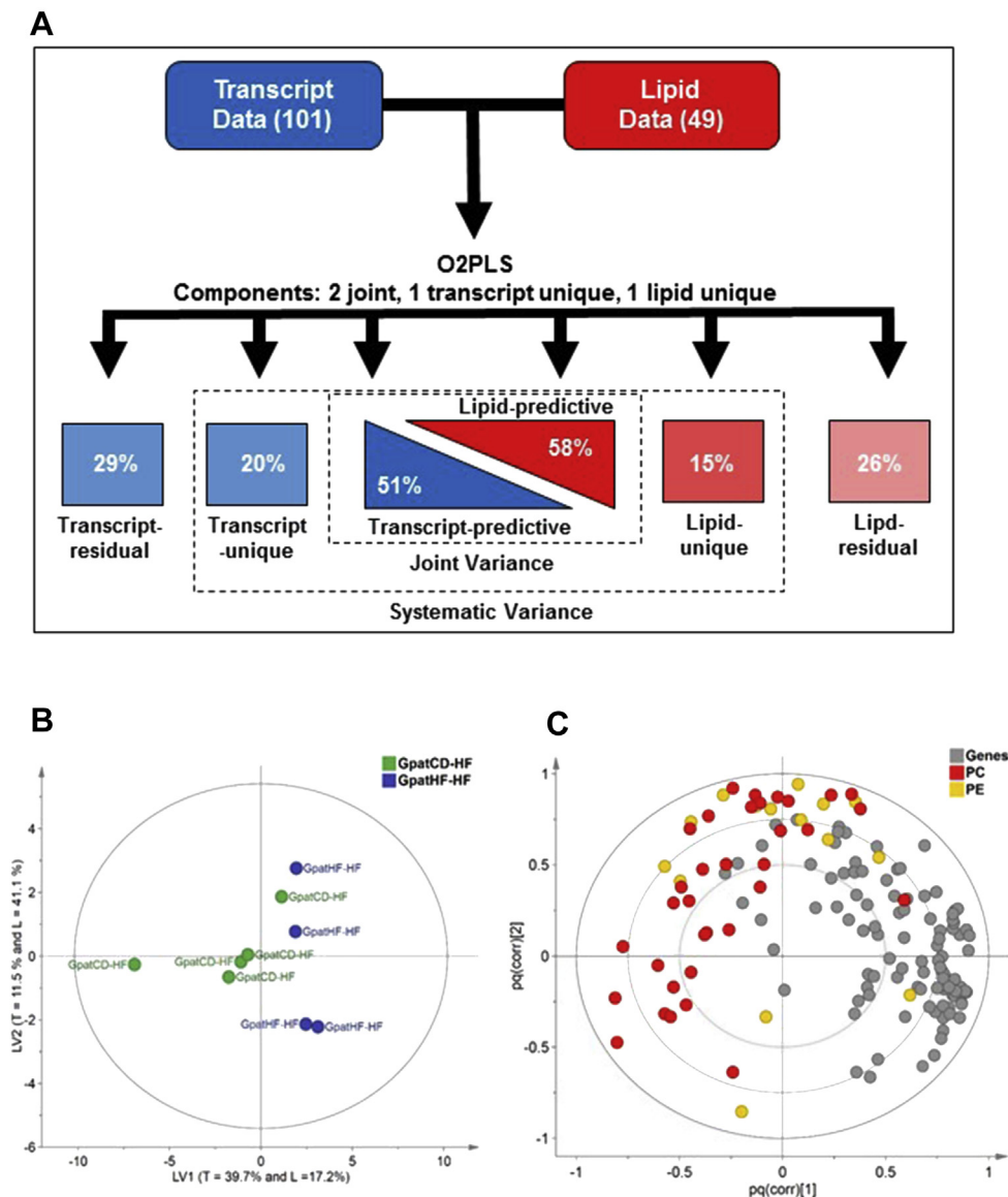
Figure 5: Enriched UPR is associated with increased phosphatidylcholine levels. A ) Overview of O2PLS model representing the UPR gene set (101 genes) from the transcriptomic data and the phosphatidylcholine and PE lipid species from the lipidomic data of EDL from F2 female rats. Total joint variance shows 51% variance for the transcript analysis of the UPR data set and 58% variance for the lipidomic data including only phosphatidylcholine and phosphatidylethylamine lipid species. The transcript-unique variance and the lipid-unique structures reached 20% and 15% variance, respectively. Residual data are 29% and 26% for the transcriptomic and lipidomic data sets, respectively. B ) O2PLS score plot of the two joint latent variables. Joint latent variable (LV) 1 accounts for 40% and 17% of the transcriptomic (T) and lipidomic (L) data sets, accordingly. The joint latent variable 2 accounts for 12% and 41% of the transcriptomic and lipidomic data sets. C ) Loading plot for O2PLS in B, consisting of 101 genes, 34 phosphatidylcholine and 15 phosphatidylethylamine species. The loadings are scaled as a correlation coefficient ranging from -1 to 1 ( n = 150 variables). GpatCD-HF: HFD-fed offspring from grandfathers fed chow diet; GpatHF-HF: HFD-fed offspring from grandfathers fed HFD.
