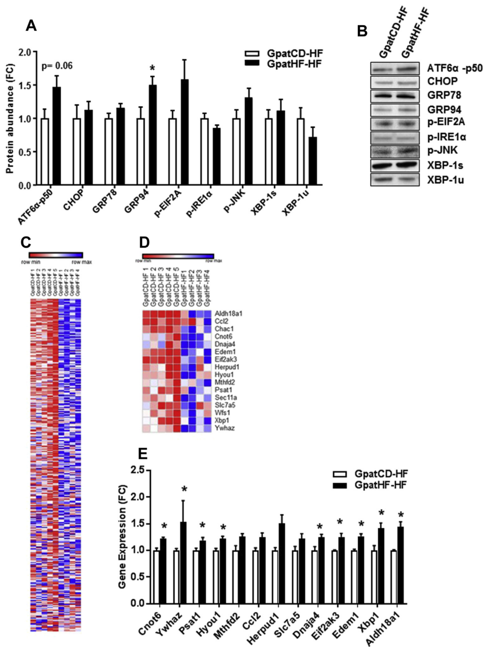
Figure 3: Activation of the ATF6 pathway in skeletal muscle of F2 female rats from HFD-fed grandfathers. A) Protein abundance of ATF6 \alpha -p50, CHOP, GRP78, GRP94, p-EIF2A, p-IRE1 \alpha , p-JNK, unspliced XBP1(u), and spliced XBP1(s) in EDL muscle of F2 rats. Data are represented as fold change (FC) ( n = 7-10 ). B) Representative blots of protein abundance of targets shown in A . C) Heatmap showing downstream targets of ATF6 \alpha retrieved from the transcriptome analysis of GpatHF-HF vs GpatCD-HF animals ( n = 4-5 ). D) Heatmap showing the downstream targets of ATF6 \alpha found in the core enrichment of the UPR gene set in GpatHF-HF vs GpatCD-HF animals ( n = 4-5 ). Red: downregulation; Blue: upregulation. E) Expression of ATF6 \alpha downstream targets in the core enrichment of the UPR gene set retrieved from the transcriptome analysis of F2 rats ( n = 4-5 ). * p \leq 0.05 : GpatHF-HF vs. GpatCD-HF. GpatCD-HF: HFD-fed offspring from grandfathers fed chow diet; GpatHF-HF: HFD-fed offspring from grandfathers fed HFD.
