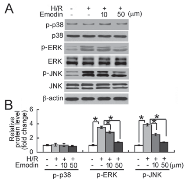
Figure 4. Emodin inhibits H/R-induced activation of MAPK signaling. HK-2 cells were pretreated with or without emodin 2 h before exposure to H/R and subjected to western blot analysis to determine the effects on MAPK signaling. (A) Representative western blots showing the expression and phosphorylation status of MAPKs (JNK, ERK and p38) are shown. (B) Densitometric analysis of p-ERK, p-JNK and p-p38 MAPKs. Data are representative of three independent experiments. * P < 0.05 . H/R, hypoxia/reoxygenation; HK-2, human renal tubular cell line; MAPK, mitogen-activated protein kinase; JNK, c-Jun N-terminal kinase; ERK, extracellular signal-regulated kinase; p-, phosphorylated.
