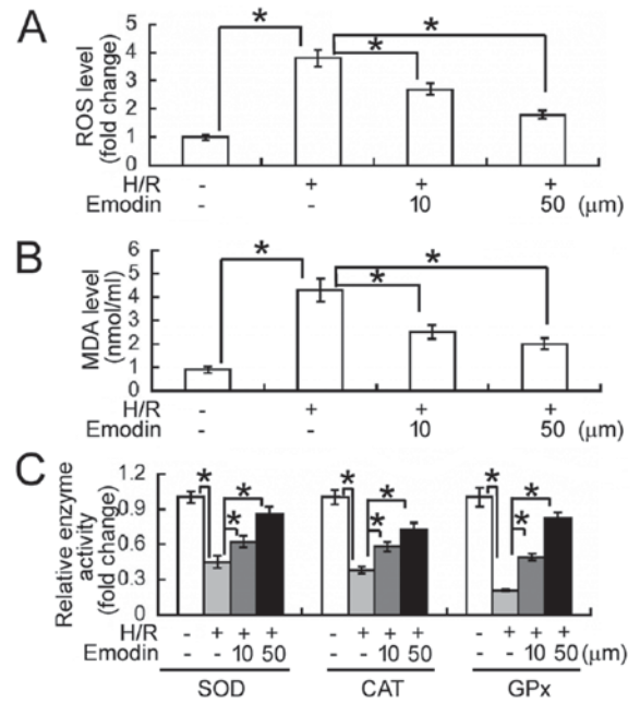
Figure 3. Emodin alleviates oxidative stress in HK-2 cells following H/R. Cells were pretreated with or without emodin 2 h before exposure to H/R and levels of oxidative stress were evaluated. The levels of (A) ROS and (B) MDA and the activities of (C) antioxidant enzymes (SOD, CAT and GPx) were measured. Data are representative of three independent experiments. * P < 0.05 . H/R, hypoxia/reoxygenation; HK-2, human renal tubular cell line; ROS, reactive oxygen species; MDA, malondialdehyde; SOD, superoxide dismutase; CAT, catalase; GPx, glutathione peroxidase.
