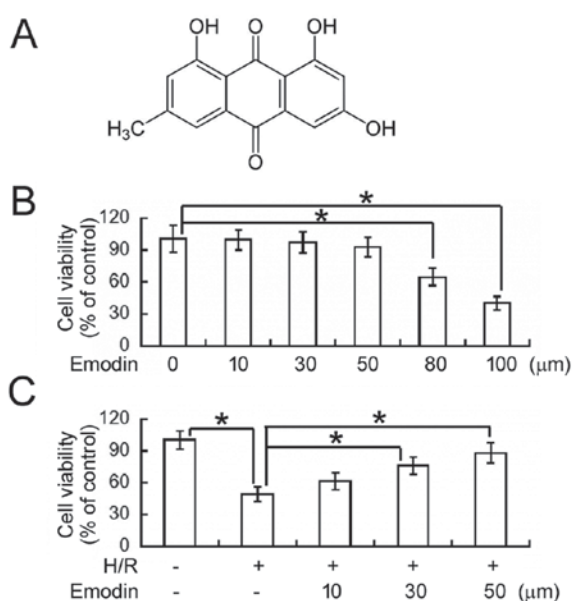
Figure 1. Emodin alleviates H/R-induced cellular damage in HK-2 cells. (A) Chemical structure of emodin. (B) Cytotoxicity of emodin in normoxic HK-2 cells was determined by an MTT assay following exposure to different concentrations of emodin for 48 h. (C) Measurements of the viability of H/R-exposed HK-2 cells with or without emodin pre-treatment. Data are representative of three independent experiments. * P < 0.05 . H/R, hypoxia/reoxygenation; HK-2, human renal tubular cell line.
