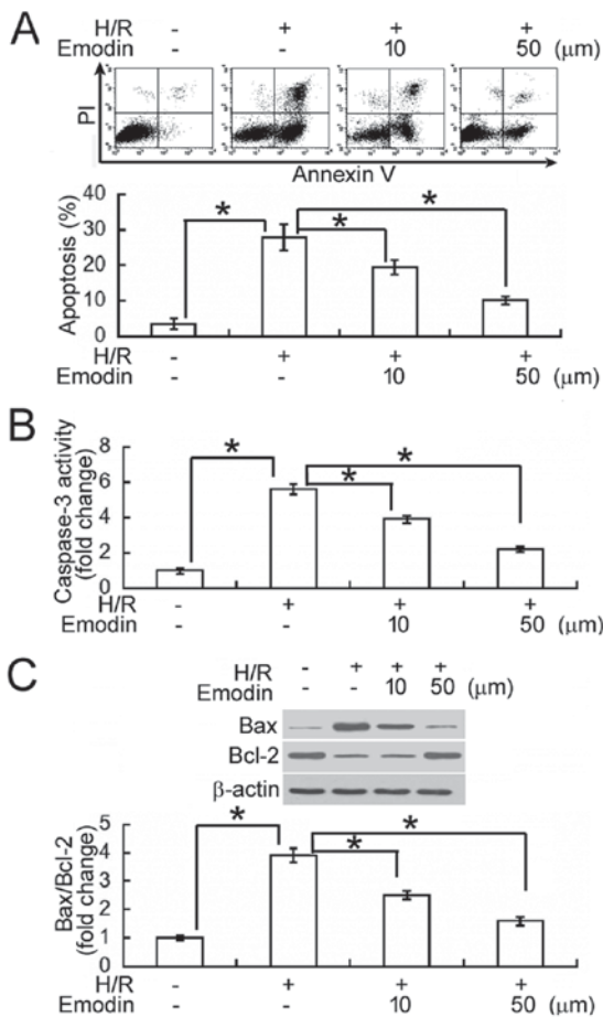
Figure 2. Emodin prevents H/R-induced apoptosis in HK-2 cells. HK-2 cells were pretreated with or without emodin 2 h before exposure to H/R and apoptotic changes were evaluated. (A) The rate of cell apoptosis was measured by flow cytometry following Annexin-V/PI staining. The lower and upper right quadrants show the proportions of early (Annexin V + /PI - ) and late (Annexin V + /PI + ) apoptotic cells, respectively. (B) Measurements of caspase-3 activity as an indicator of apoptosis. Results are expressed as the fold change in activity relative to normoxic cells. (C) Western blot analysis of Bax and Bcl-2 protein expression. Representative western blots are shown. Bax/Bcl-2 ratios were determined from immunoblotting data. Data are representative of three independent experiments. * P < 0.05 . H/R, hypoxia/reoxygenation; HK-2, human renal tubular cell line; PI, propidium iodide; Bcl-2, B-cell lymphoma-2; Bax, Bcl-2-associated X protein.
