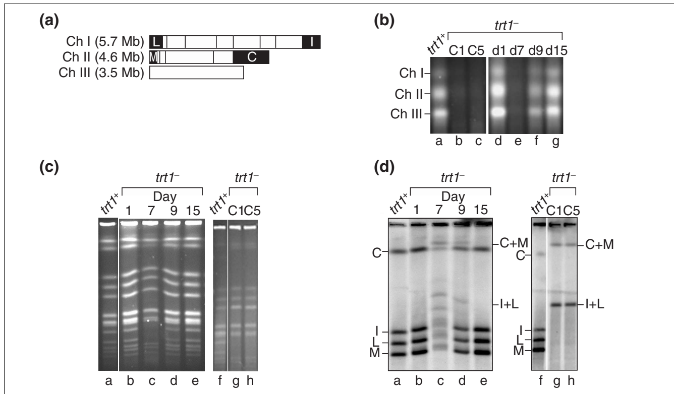
Figure 3 Chromosome structures of trt1 - survivors. (a) The 13 NotI restriction sites in S. pombe chromosomes I and II [65] are indicated by vertical lines. Chromosome III does not have a NotI site. Terminal fragments are labeled according to convention and highlighted in black. (b) Pulsed-field gel analysis of intact chromosomes visualized by staining with ethidium bromide. Lanes d-g correspond to days 1, 7, 9 and 15 of the growth curve, respectively. (c) Pulsed-field gel of NotI -digested chromosomes visualized with ethidium bromide. Days 1, 7, 9 and 15 correspond to days of the growth curve. Lanes a and f were repositioned from the original gel image. (d) The gels from (c) were transferred to a nylon membrane and probed with a mixture of 32 P-labeled probes to internal regions of the C, I, L and M fragments, identified in (a). The terminal fragments of linear chromosomes are labeled on the left, and fragments C+M and I+L resulting from circularized chromosomes are shown on the right.
