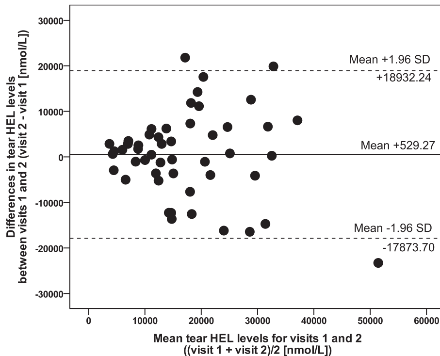
FIGURE 1. Bland-Altman plot illustrating variability of raw data for tear HEL levels ( n = 50 ). Solid line shows bias (mean differences). Dotted lines show 95% limits of agreement.
