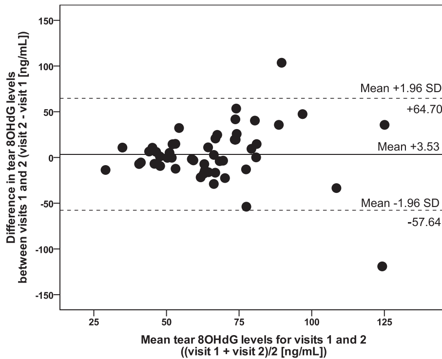
FIGURE 2. Bland-Altman plot illustrating variability of raw data for tear 8OHdG levels ( n = 50 ). Solid line shows bias (mean differences). Dotted lines show 95% limits of agreement.
