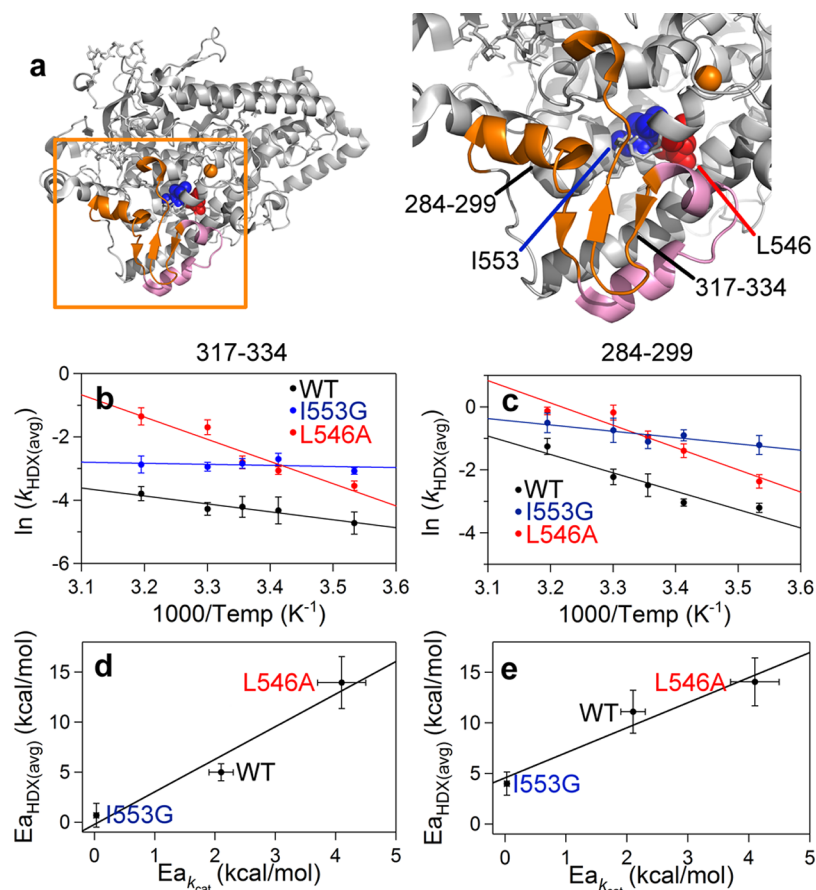
Figure 4. Peptides (in orange) remote from the active site that exhibit mutation-induced changes in the enthalpic barrier for HDX rates ( E_{a\text{HDX}(\text{avg})} ) (a). The enzyme structure is shown rotated 180^\circ relative to Figure 2a. The pink colored peptides (297–305 and 306–316) have altered rates of exchange, but the E_{a\text{HDX}(\text{avg})} values are the same for all SLO-1 variants (Figure S8 and Table S5). Peptides displayed in orange, 317–334 (b and d) and 284–299 (c and e) are those that exhibit mutant variable E_{a\text{HDX}(\text{avg})} . In panels b and c, Arrhenius-like plots of the weighted average exchange rates, \ln(k_{\text{HDX}(\text{avg})}) , for WT, I553G, and L546A are compared. The HDX traces for these peptides are found in Figure S7. In panels d and e, the relationship between E_{a\text{HDX}(\text{avg})} and the enthalpic barrier for hydrogen tunneling ( E_a(\text{H}) ) is shown.
