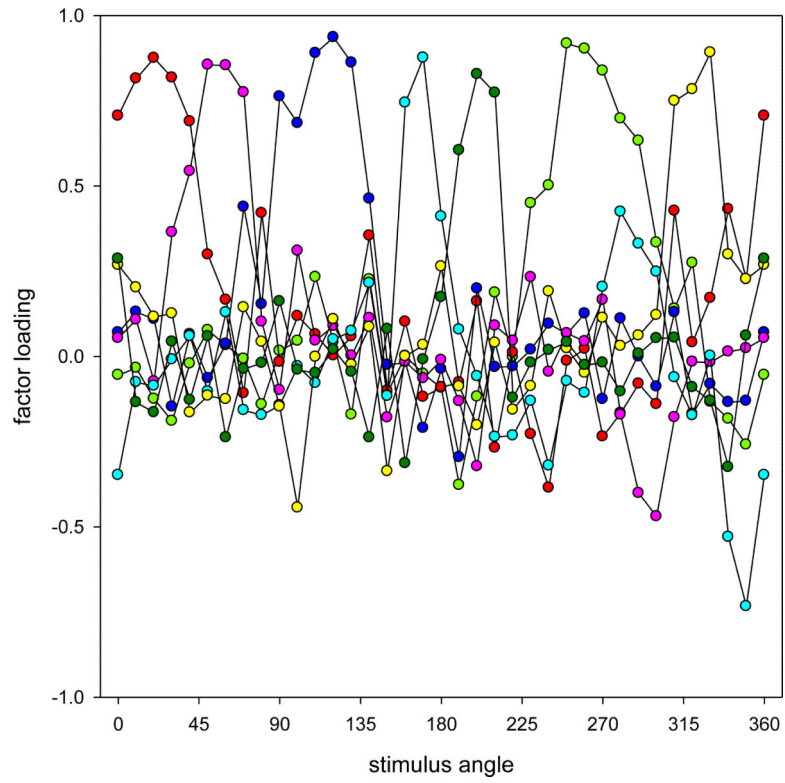
Figure 2. Factor loadings for the hue scaling functions (new data set). Curves show the loadings for the seven systematic factors following Varimax rotation.
