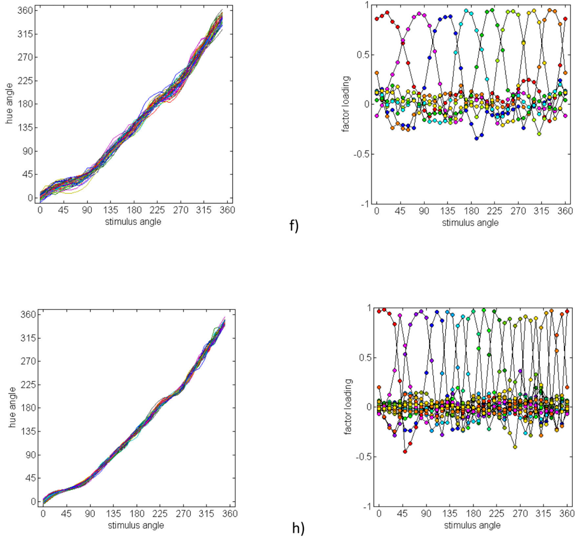
Figure 7. Predicted scaling functions and factors based on a population code for color with varying anchors corresponding to the stimulus angles associated with different hues. a) and b) Simulated scaling functions and factor loadings based on four variable anchors centered on the four primary hues. c) and d) Predictions for eight anchors corresponding to the focal angles for the unique or binary hues. e) and f) Eight anchors with added measurement noise. g) and h) Sixteen anchored hues.
