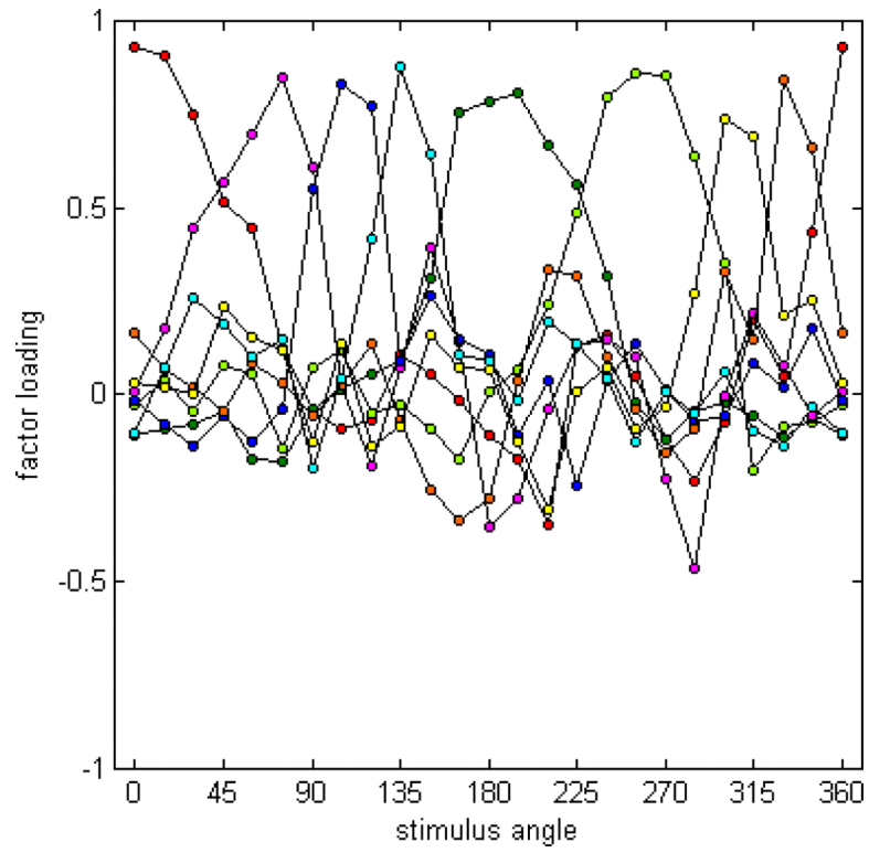
Figure 3. Factor loadings for the hue scaling functions of Malkoc et al. (2005). Plotted are the eight factors showing systematic loadings following Varimax rotation.
