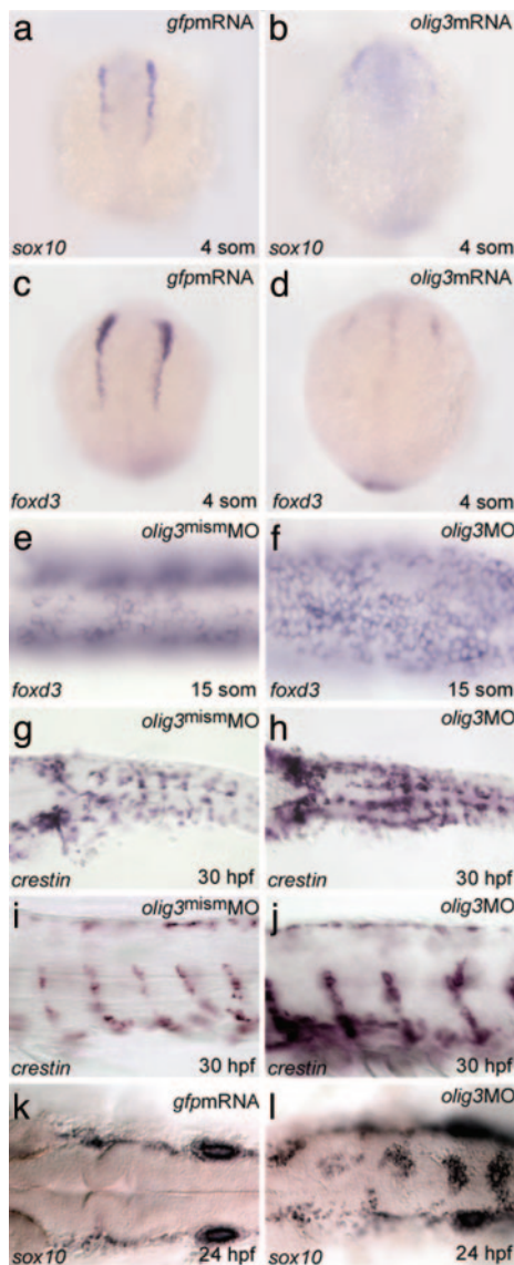
Fig. 2. olig3 controls specification of the neural crest. (a–d) The levels and the expression domains of sox10 and foxd3 are decreased in four-somite embryos injected with olig3 mRNA (b and d) (phenotype in >90% of injected embryos, n = 30). (e and f) The expression of foxd3 is increased in 15-somite embryos treated with olig3 MO (f) (morphant phenotype > 90%, n = 20). Similarly, the expression of crestin is increased in 30-hpf embryos treated with olig3 MO (h and f) (morphant phenotype > 90%, n = 40). Similar results are obtained in 24-hpf embryos hybridized with sox10 (k and l) (morphant phenotype > 90%, n = 30). Embryos are in dorsal (a–h, k, and l) or lateral (i and j) view, anterior to the top (a–d) or to the left (e–l).
