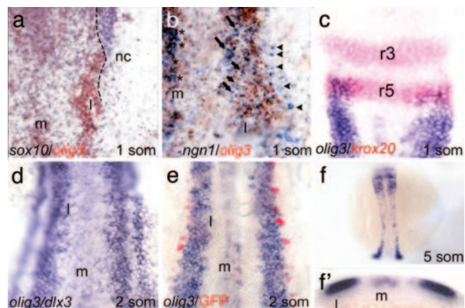
Fig. 1. olig3 expression pattern. (a) High magnification of the right side of the rhombencephalon region showing that olig3 (brown) is expressed medially to the neural crest marker sox10 (blue); the dashed line represents the boundary of expression of the two markers. (b) High magnification of the right side of the trunk region shows that the lateral (l) olig3 (brown) expression domain comprises the region where ngn1 -positive interneurons (arrows) differentiate. RB cells (arrowheads) are in a more lateral position and are outside the olig3 expression domain. (c) The anterior border of the olig3 domain (blue) is delimited by krox20 (red) in rhombomere-5 (r5). (d) The olig3 domain has elongated rostrocaudally, and a two-cell-wide gap separates olig3 and dlx3 . (e) ngn1 :GFP transgenics showing that RB-cell precursors (red) and olig3 -expressing cells are in close contact. (f) At the five-somite stage, the lateral domain has further elongated. (f') Transverse section at the level of the posterior trunk of the embryo in f . The embryos are in dorsal view, anterior to the top.
