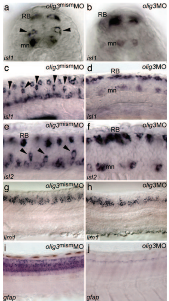
Fig. 3. olig3 knockdown affects differentiation of lateral neural plate cells. (a–f) islet1/2 -expressing interneurons (a and b; black arrowheads in a) (18, 19) are absent in 20-somite (b and d) and 24-hpf (f) embryos injected with olig3 MO. Conversely, RB cells (RB) are increased in number in olig3 morphants (b, d, and f) (morphant islet1 -phenotype > 90%, n = 40; morphant islet2 -phenotype > 90%, n = 30). mn, motoneurons. (g and h) lim1 is expressed at 24 hpf in D3 interneurons of the dorsal spinal cord (g). D3 interneurons are slightly affected in embryos injected with olig3 MO (h) (morphant phenotype > 90%, n = 15). (i and j) The glial fibrillar acidic protein gene ( gfap ) is expressed at 3 days postfertilization in astrocytes of the dorsal spinal cord (i). gfap expression is absent in embryos injected with olig3 MO (j) (morphant phenotype > 90%, n = 20). Embryos are in transverse sections (a and b) or in lateral view with anterior to the left (c–j).
