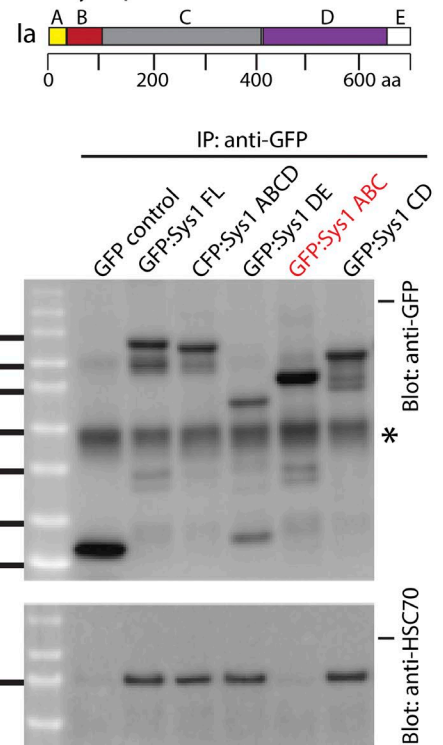
Figure 4. Characterization of synapsin protein complexes from nonsynaptosomal fractions. (A) Functional categorization of peptides identified in the non-synaptosomal (P100 and S100) fractions (“%” represents number of proteins in the functional group per total number proteins in the fraction \times 100). (B) Bar graphs showing raw spectrum counts for selected chaperones detected in the S100 fraction. Error bars show means \pm SEM. (C) Protein-protein interaction map of the chaperones identified in the S100 fraction. Individual proteins are highlighted by red dots, and protein-protein interactions are indicated by light gray lines. The dashed circle highlights the Hsp peptides. (D) CoIP of synapsin and Hsc70 in HEK293T cells. HEK cells were either transfected with the full-length GFP-tagged synapsin or various GFP-tagged deletion mutants containing only some of the domains that make up the protein (a schematic of various synapsin domains is on top). The transfected synapsin and endogenous Hsc70 was detected by anti-GFP and anti-Hsc70 antibodies, respectively. Note that only the synapsin deletion lacking the D-domain failed to associate with Hsc70 (fifth lane from left, bottom gel). The asterisk indicates IgG heavy chain. Molecular mass is indicated in kilodaltons.
