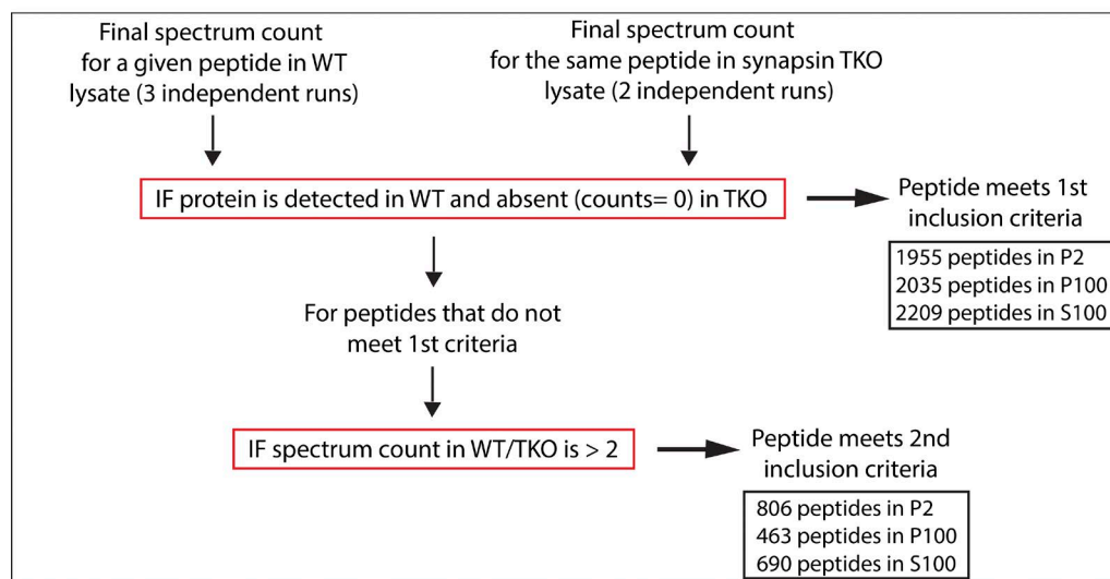
Figure 2. Criteria for including synapsin-interacting peptides identified by MudPIT-MS analysis. Raw spectrum counts for a given protein from WT and TKO lysates were normalized and averaged to obtain final spectral counts using conventional strategies as detailed in the Isolation of synapsin complexes... section of Results. The following inclusion criteria were then applied to determine synapsin-associated proteins. First, peptides detected in WT but not in the TKO lysates (spectrum count = 0) were included. Second, peptides with final spectrum counts of twofold or more than TKO fractions were also included in the list. The final numbers of proteins are indicated in the black boxes. IF, immunofluorescence.
