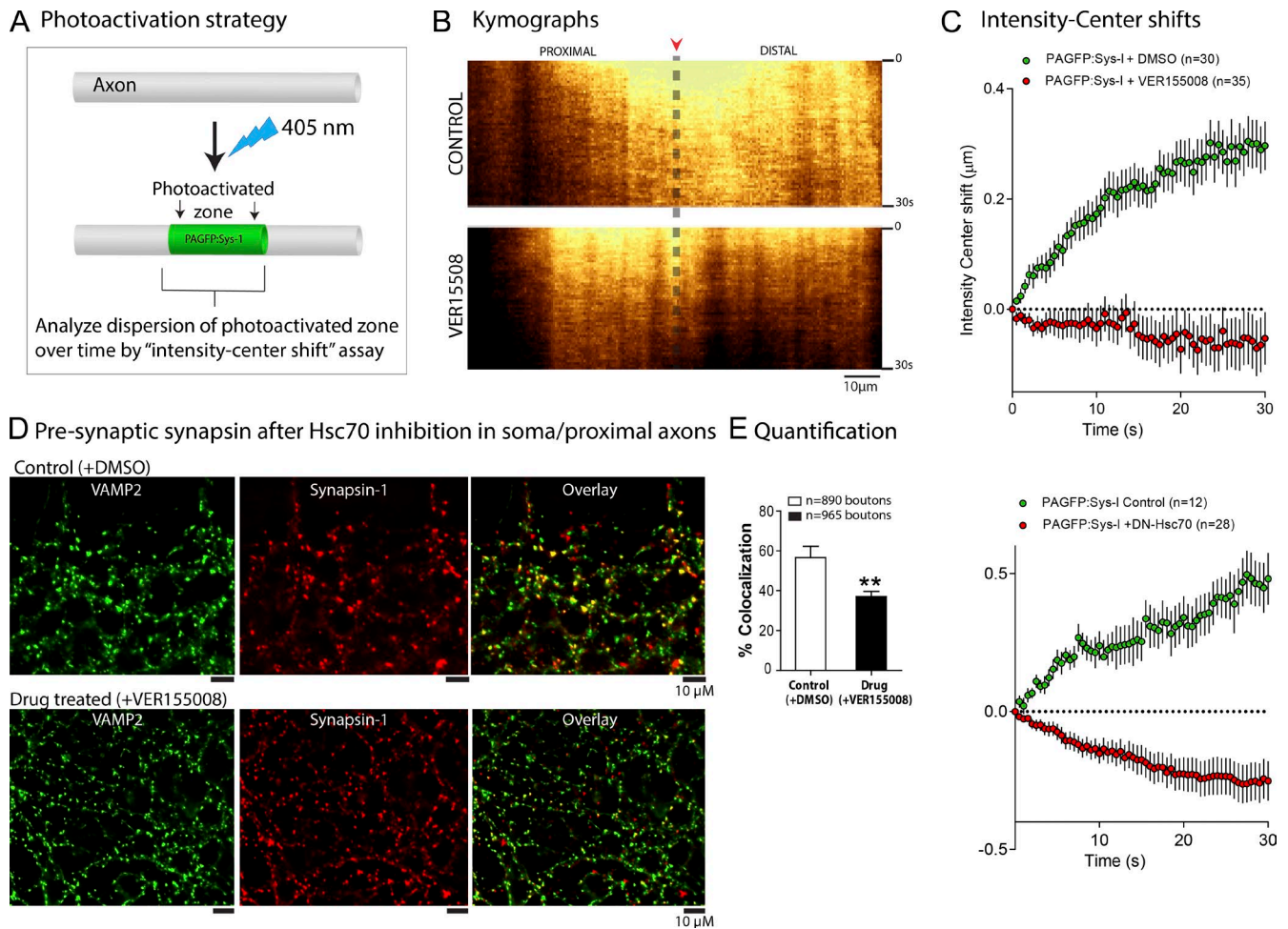
Figure 6. Inactivation of Hsc70 ATPase activity blocks slow axonal transport and presynaptic accumulation of synapsin. (A) Schematic of assay to determine slow axonal transport of synapsin using photoactivatable synapsin (PAGFP:synapsin; Roy et al., 2011; Scott et al., 2011). In brief, PAGFP:synapsin was photoactivated in a discrete axonal ROI, and the fluorescence was tracked over time by live imaging. (B) Kymographs from photoactivation experiments in A. Note the anterogradely biased dispersion of PAGFP:synapsin fluorescence in control axons, thought to represent slow transport (midpoint of photoactivated zone marked by red arrowhead and dashed line; top). Also note that the Hsc70 inhibitor (100 \mu M VER155008; bottom) eliminated the anterograde bias. (C) Quantification of the transport experiments. In brief, the centroid of the photoactivated zone was quantified in each image of a given time-lapse video, and the displacement of the centroid was quantified over time (intensity center shift; Scott et al., 2011). Note that although the population of photoactivated synapsin was transported anterogradely, pharmacologic (VER155008) or genetic (DN-Hsc70) inactivation of Hsc70 ATPase activity prevented the biased transit. (D) Attenuation of endogenous synapsin levels at presynaptic boutons upon selective inactivation of Hsc70 in axons. Axons and presynaptic boutons were isolated from somatodendritic compartments using a triple-chamber microfluidic device (see Fig. S1 for design of device). Thereafter, the Hsc70 inhibitor VER155008 (or DMSO control) was selectively added to the axonal/presynaptic chamber, and the neurons were fixed and immunostained with anti-VAMP2 (to detect all presynapses; green) and anti-synapsin (red) antibodies. Representative images from axonal/presynaptic chambers are shown. (E) Quantification of colocalization between synapsin and VAMP2. Note that Hsc70 inactivation significantly attenuated the presynaptic localization of synapsin. Error bars show means \pm SEM. **, P < 0.01 .
