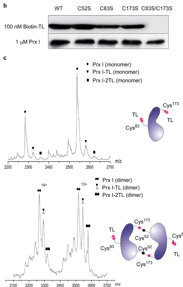
Fig. 2 Structural characterization of Prx I-TL and confirmation of the binding sites. (a) MS/MS analysis of the Cys 173 -containing tryptic peptide after recombinant Prx I was incubated with TL, followed by trypsin digestion. The asterisk indicates the residue bound by TL; red labels show ions that display a mass shift corresponding to TL. (b) 1 \mu\text{M} recombinant Prx I and its mutants were incubated with 100 nM Biotin-TL at 4 ^{\circ}\text{C} for 3 h, followed by Western blotting for biotin or Prx I. (c) Native ESI-MS analysis of the monomer (upper) and dimer (lower) of the Prx I-TL complex. 10 \mu\text{M} recombinant Prx I was incubated with vehicle or 40 \mu\text{M} TL at 4 ^{\circ}\text{C} overnight before analysis. Schematic diagrams show interactions between TL and the Prx I monomer/dimer.
