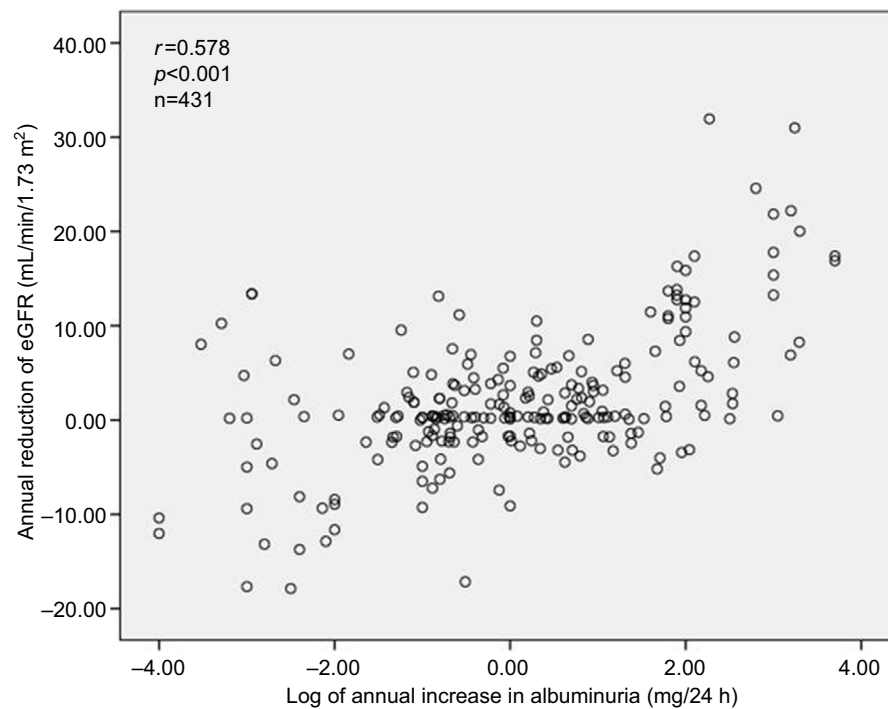
Figure 2 Annual reduction plot of eGFR versus annual increase in albuminuria.
