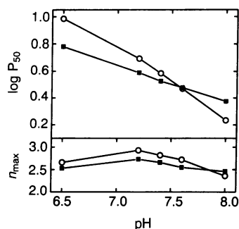
FIG. 6. Oxygen-binding properties of recombinant Hb (■) and human Hb A 0 (○). P 50 values and Hill coefficients ( n_{\max} ) were obtained in 50 mM Hepes buffer/0.1 M NaCl, 25 ± 0.1°C, at pH 6.5, 7.2, 7.4, 7.6, and 8.0.
