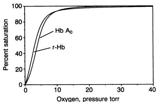
FIG. 5. Oxygen equilibrium curves comparing recombinant Hb (r-Hb) and Hb A_0 in 50 mM Hepes, pH 7.4/0.1 M NaCl at 25 \pm 0.1^\circ\text{C} . (1 torr = 133 Pa.)
