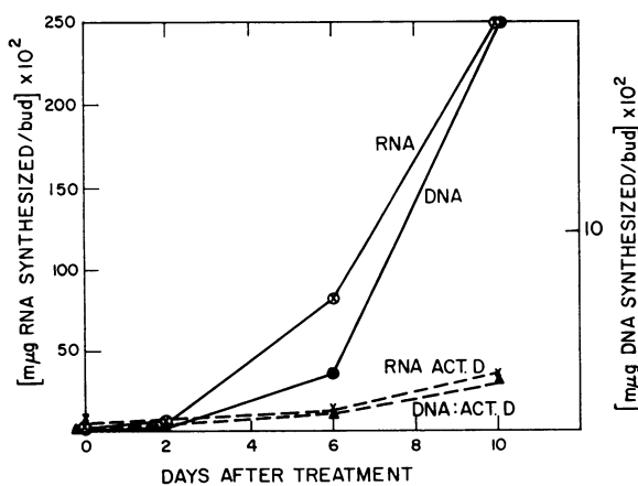
FIG. 2. Rate of incorporation of the carbon of uridine-2-C 14 into RNA and DNA by buds of potato tubers at varying times after 3-day pretreatment with ethylene chlorohydrin. In the 2 lower curves of figure 2, the buds were incubated in solution containing not only uridine-2-C 14 , but also actinomycin D.
