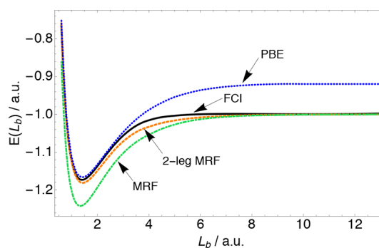
Figure 4. H_2 molecule dissociation curve as a function of the internuclear distance L_b/a.u. obtained with the MRF-1 and 2-leg MRF approaches presented in this work, compared to restricted PBE and FCI. All the curves have been obtained using the aug-cc-pCVTZ basis set. 56
