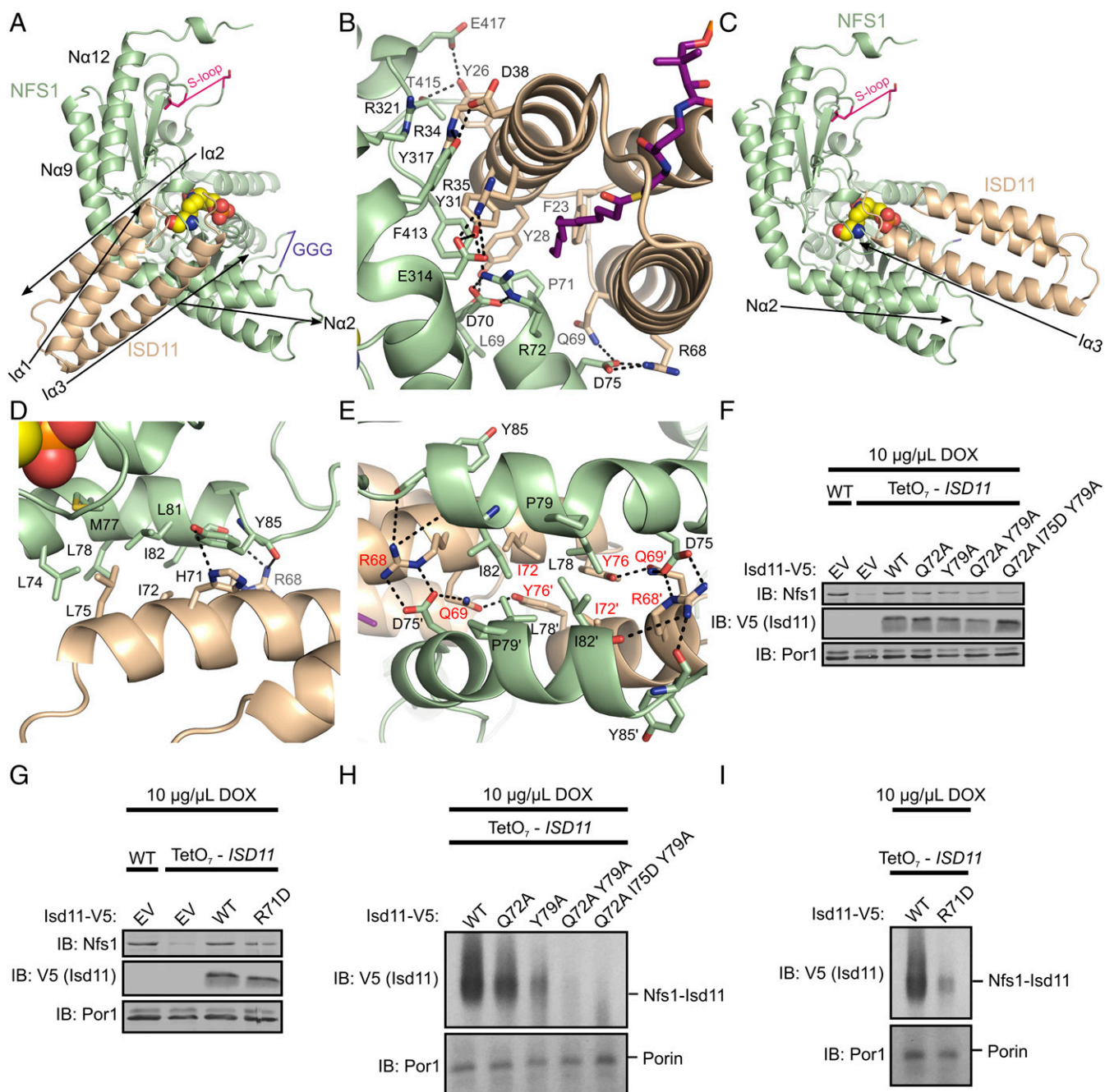
Fig. 3. Two distinct NFS1–ISD11 interfaces are important for forming the SDA_{ec} architecture. (A) Global overview of the primary NFS1–ISD11 interface (ACP and lipid are omitted for clarity). ISD11 packs against N\alpha 9 , N\alpha 12 , and N\alpha 2 helices of NFS1. (B) Specific interactions of the primary NFS1–ISD11 interface (ACP omitted for clarity). The acylated 4'-PPT is shown in purple. (C) Global overview of the secondary NFS1–ISD11 interface. ISD11 \alpha 3 has an antiparallel orientation compared with NFS1 N\alpha 2 . (D) Specific interactions of the second NFS1–ISD11 interface. The PLP is shown in spheres. (E) The 4-helix bundle core of the SDA_{ec} complex. Residues labeled in red were tested in vivo using analogous substitution in S. cerevisiae . Arrows show the polypeptide direction for the \alpha -helices. Purified mitochondria from the indicated strains were solubilized from cells similar to Fig. 2 and resolved by SDS/PAGE (F and G) and BN-PAGE (H and I). EV, empty vector; IB, immunoblot.
