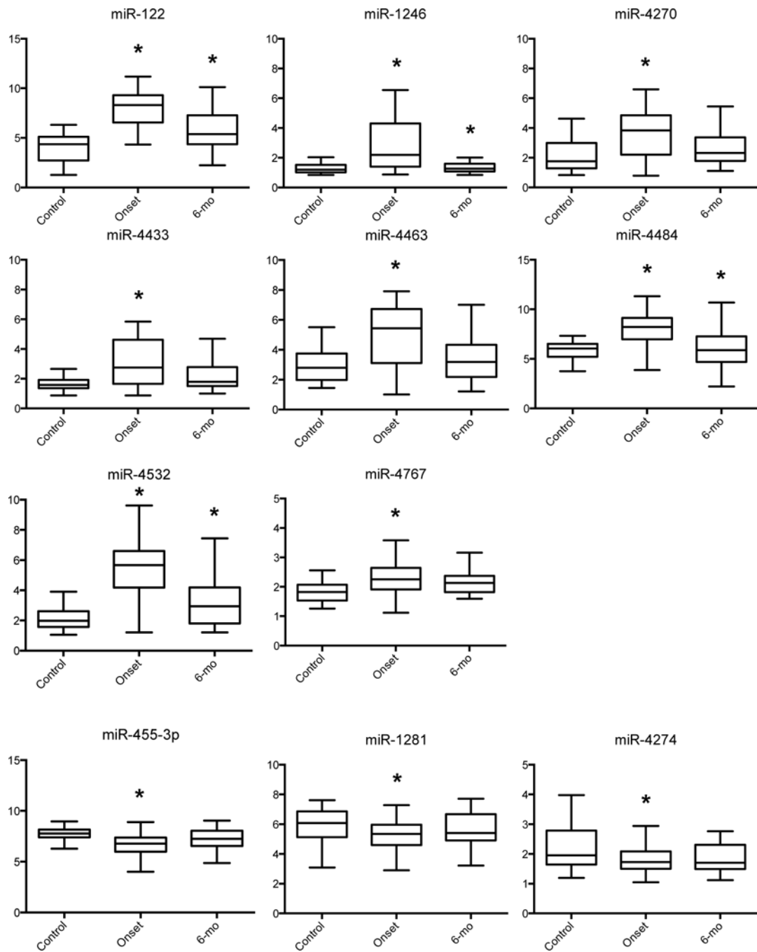
Figure 3. miRNA Concentrations differentially distributed among DILI onset and 6 month follow-up. Y axis is fold change
