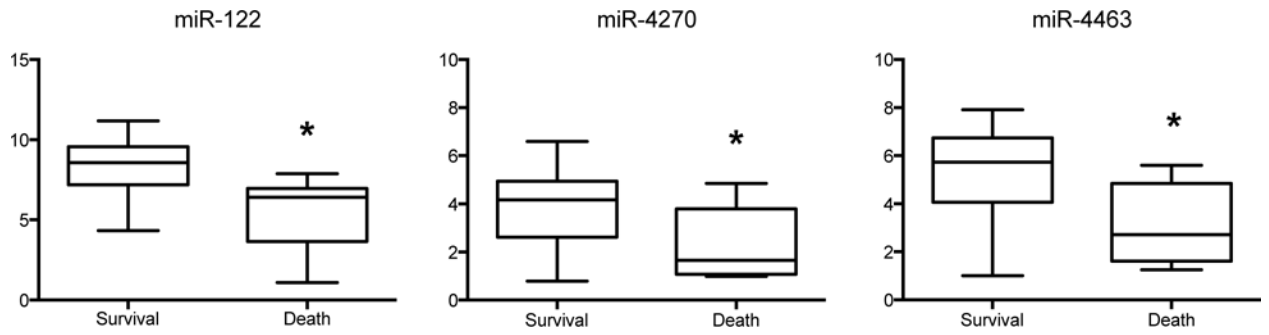
Figure 4. Values for miR-122 among those who survived (n=68) vs died (n=10) within 6 months of DILI onset. Results are expressed as in Fig. 3. Y axis is fold change.
