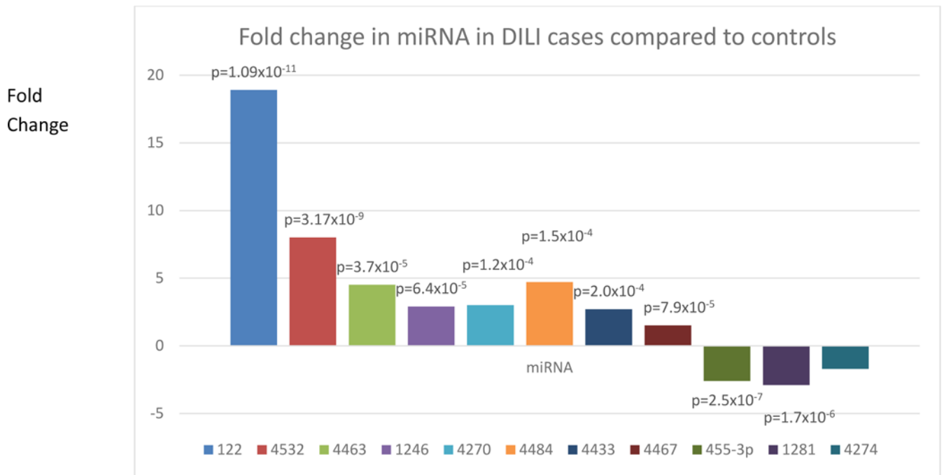
Figure 2. miRNA Levels in Serum for Subjects with Acute DILI, expressed as Fold-Difference from Those for Control Subjects. Y axis is fold change
