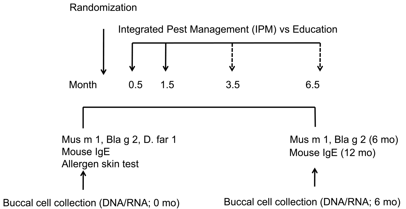
Figure 1. Study algorithm
