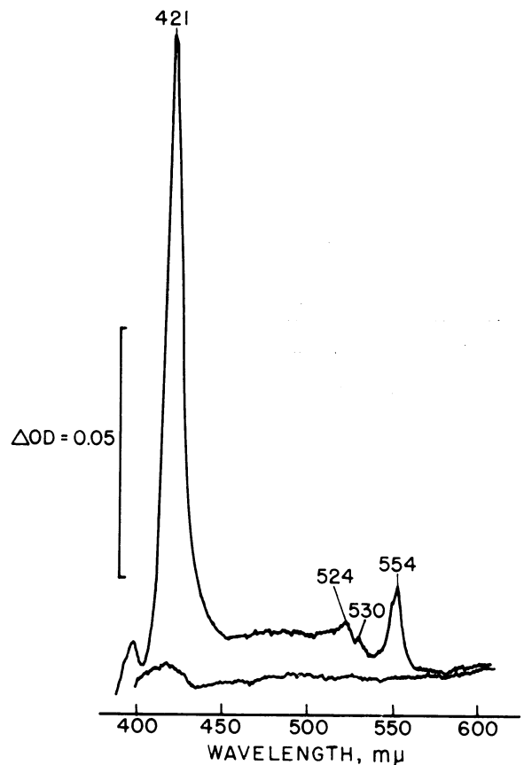
FIG. 2. Chloroplast lamellar protein fraction. Difference spectrum, untreated minus oxidized ( 2 \times 10^{-5} M ferricyanide), obtained using split compartment cuvettes. The lower curve is a base line, untreated minus untreated. The upper curve was obtained by mixing the compartments of the cuvette in the reference beam and shows the absorption spectrum of cytochrome f.
