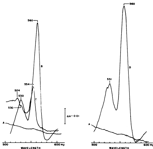
FIG. 4. Difference spectra of an 80% acetone powder of pure spinach chloroplast lamellae. Powder suspended in 0.1 M Tris-Cl, pH 8.0. A, base line. B, dithionite-reduced minus untreated. C, untreated minus ferricyanide-oxidized. D, dithionite-reduced minus ferricyanide oxidized. Solid dithionite and ferricyanide were added to the cuvettes.
