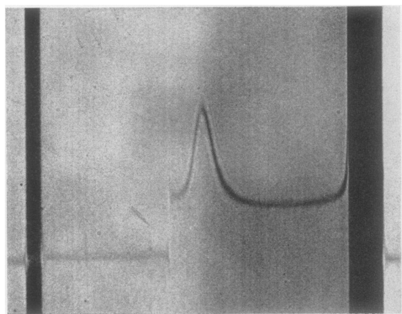
FIG. 6. Schlieren photograph of the chloroplast lamellar protein fraction during a sedimentation velocity determination. The color due to the cytochromes is clearly associated with the boundary. Protein 7 mg/ml in 0.1 M NaCl, 0.002% Na-dodecyl sulfate, 5 \times 10^{-2} M Tris, pH 8. Rotor speed 59,780 rpm, 4°. Phase plate 60°. Photograph taken 12 minutes after reaching speed.
