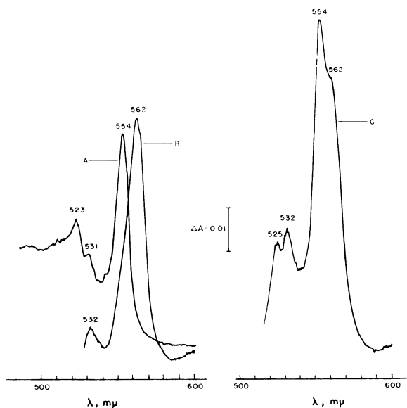
FIG. 5. Difference spectra of lipid-free chloroplast lamellae solubilized in chololate (2 mg/mg protein). A, untreated minus ferricyanide-oxidized. B, dithionite-reduced minus untreated. C, dithionite-reduced minus ferricyanide-oxidized.
