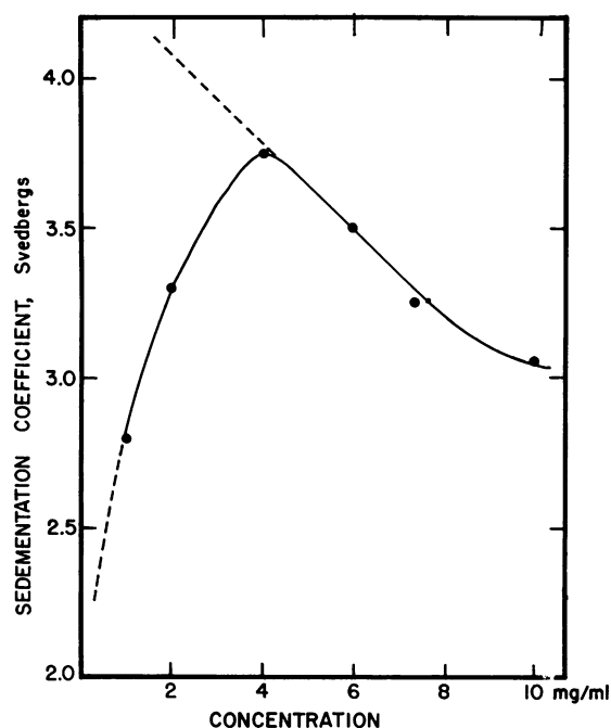
FIG. 7. Dependence of sedimentation coefficient on concentration of the lamellar protein fraction. All experiments conducted in 0.1 M NaCl, 0.002% Na-dodecyl sulfate and 5 \times 10^{-2} M Tris, pH 8.
