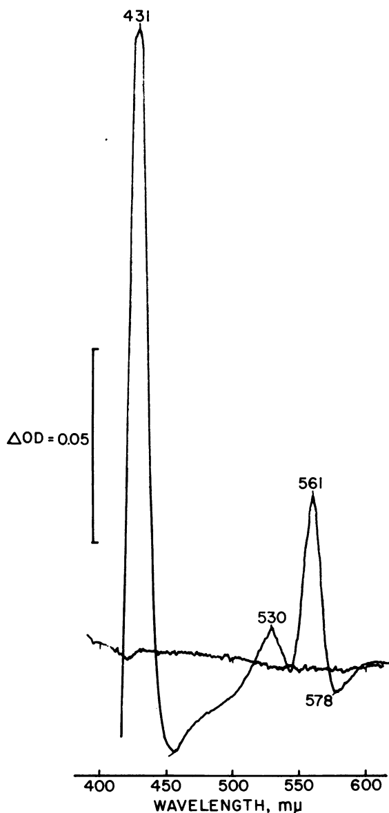
FIG. 3. Chloroplast lamellar protein fraction. Difference spectrum reduced ( 2 \times 10^{-5} M dithionite) minus untreated obtained using split compartment cuvettes. The lower curve is a base line, untreated minus untreated. The upper curve was obtained by mixing the compartments of the cuvette in the sample beam and shows the absorption spectrum of cytochrome b_6 .
