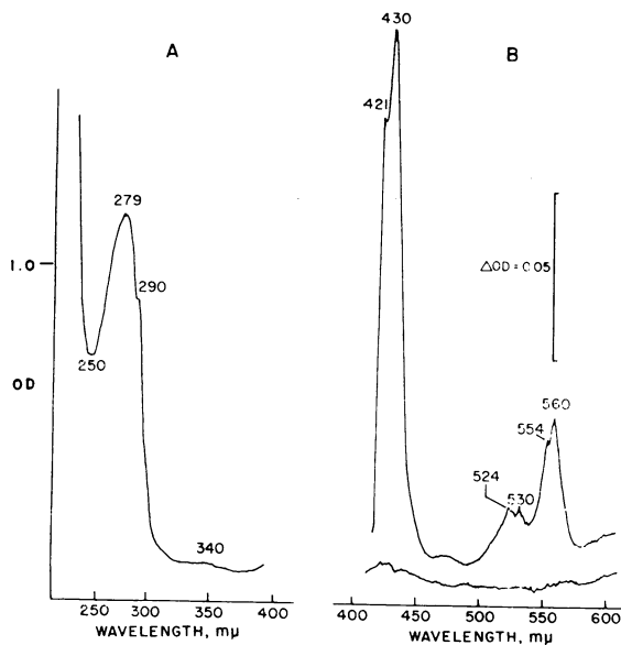
FIG. 1. Absorption spectra of the chloroplast lamellar protein fraction. A, An absolute spectrum of the ultraviolet region. B, A reduced minus oxidized difference spectrum on the same protein sample only using the 0 to 0.1 OD slide wire on the spectrophotometer. The difference spectrum was obtained using cuvettes containing protein and 10^{-4} M ferricyanide in separate compartments. The lower curve is a base line. The protein and ferricyanide in the cuvette in the reference beam was then mixed and a minute quantity of solid dithionite was added to the protein compartment of the cuvette in the sample beam.
