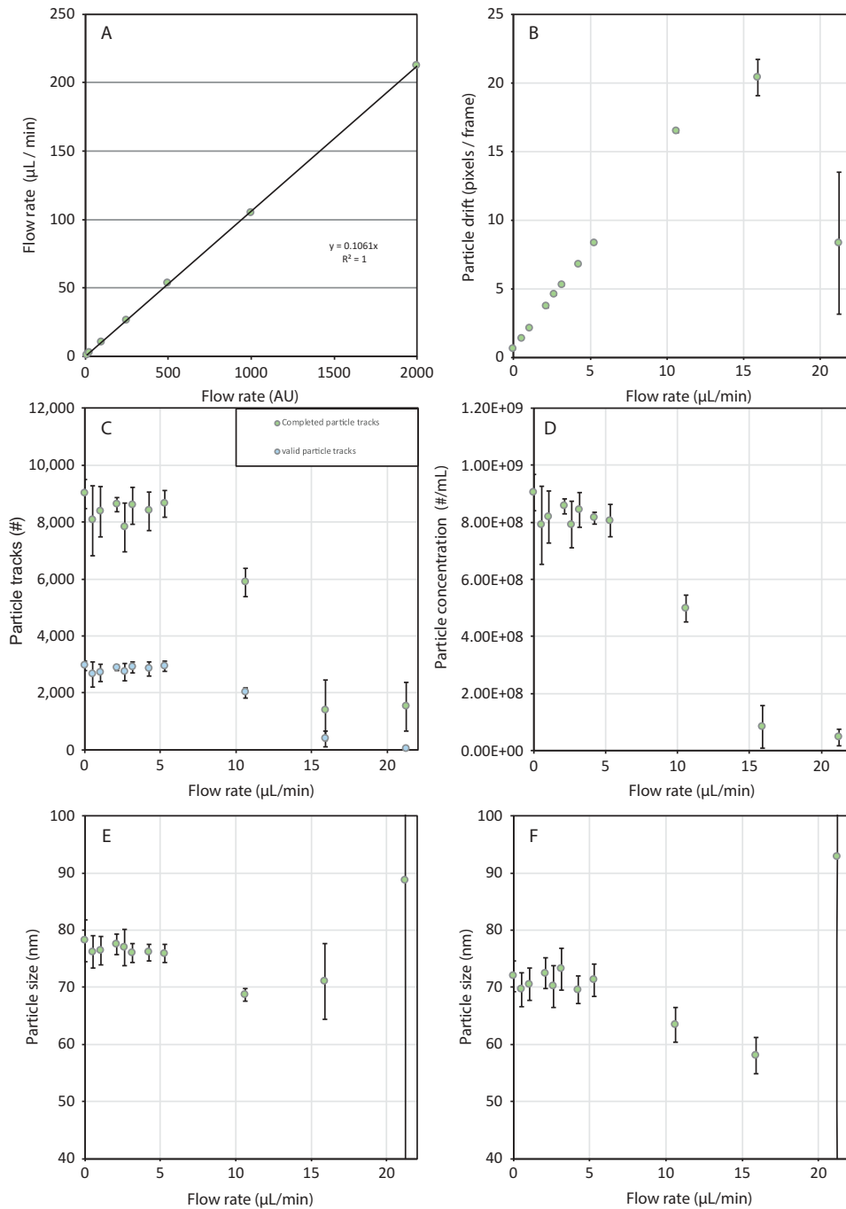
Figure 4. The influence of sample flow rate on NTA. The artificial flow rate of the NTA software has been calibrated using a 500 \mu\text{L} syringe (a). OMV stock was measured at different flow rates. The observed particle drift (b), total and valid particle tracks (c), concentration (d), mean size (e), and mode size (f) are plotted against the sample flow rate.
