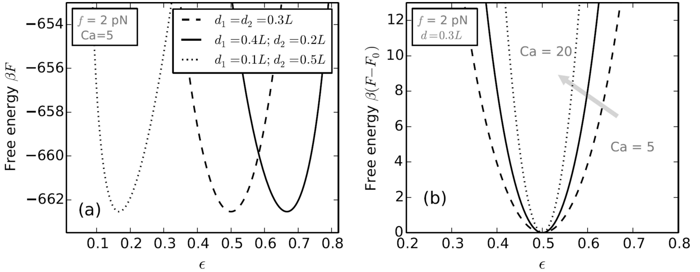
FIG. 9. Effect of the intertether distance. (a) Comparison of the free energy versus \epsilon (Eq. D.1) for braids with various choices of the two intertether distances d_1 and d_2 , but keeping the arithmetic mean of the two distances the same. The end-region where the two DNAs are closer to each other is smaller in size ( i.e. , has less DNA in it), and vice-versa. (b) Free energy versus \epsilon for braids at various catenations ( Ca=5, 12 and 20 ) with identical intertether distances d = 0.3L . The stiffness of the free energy decreases for lower catenation values indicating higher fluctuations in the relative sizes of the two end regions. The free energy curves have been shifted in the y-axis in order to overlay them.
