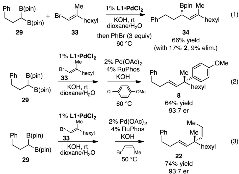
Scheme 4. Single-Flask Sequential Cross-Couplings
