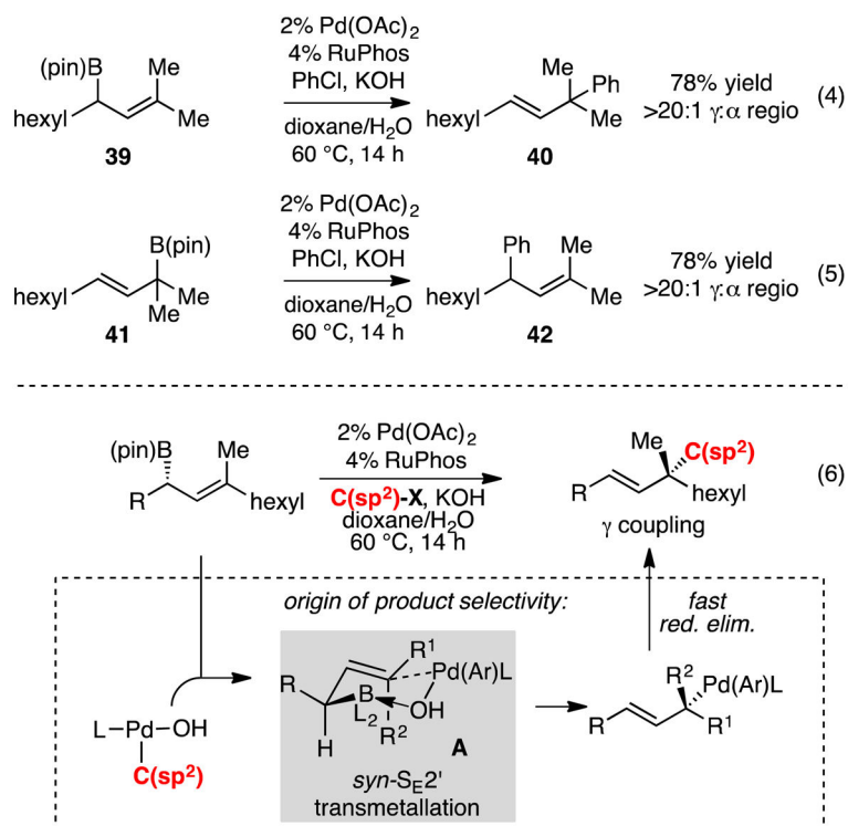
Scheme 6. Mechanistic Experiments and the Origin of Regioselectivity
