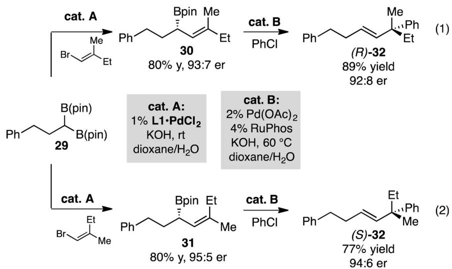
Scheme 3. Sequential Cross-Coupling to Furnish Enantiomeric Products from the Same Enantiomer of Catalyst.
