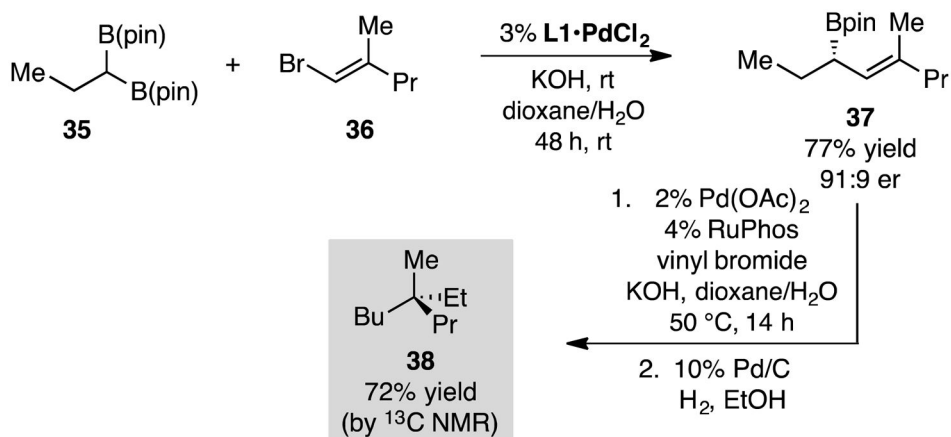
Scheme 5. Catalytic Synthesis of Chiral Hydrocarbon 38.
