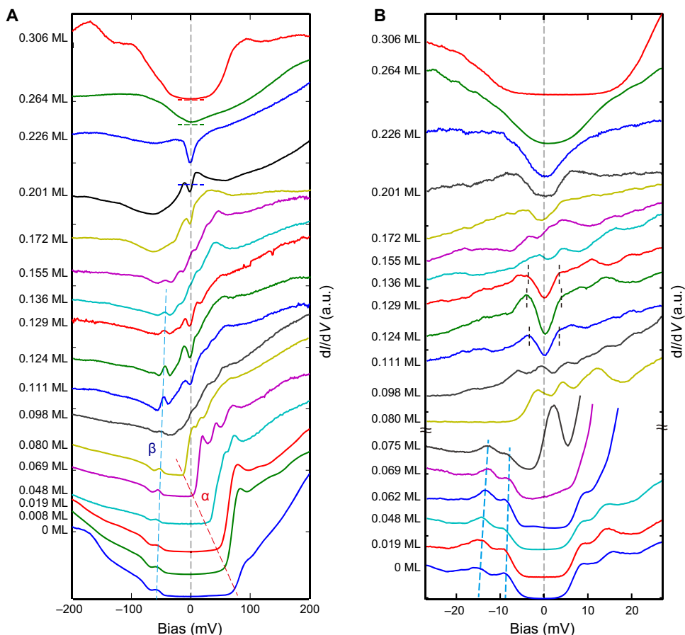
Fig. 3. Evolution of dI/dV spectra taken on the FeSe surface with various K_c as labeled. (A) Typical dI/dV spectra taken within large energy range ( \pm 200 mV). Red and blue dashed lines track the onsets of the \alpha and \beta bands. The zero positions of the spectra at K_c = 0.306 , 0.264, and 0.226 ML are marked by short horizontal bars. (B) Typical dI/dV spectra taken near E_F ( \pm 27 mV). Two blue dashed lines track the superconducting coherence peaks at negative bias. The curves at K_c \leq 0.075 ML are normalized by the dI/dV value at V_b = -27 mV, and the curves at K_c > 0.075 ML are normalized by the value at V_b = 27 mV. E_F ( V_b = 0 ) is indicated by gray dashed lines. At K_c = 0.111 , 0.124, and 0.129 ML, the gap edge positions (defined as \Delta_3 ) are marked by short dashed lines.
