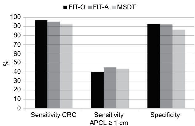
Figure 1 Sensitivity for detecting CRC and APCL ≥ 1 cm and specificity of FOB Gold (using the original cutoff) compared to Cologuard in the MSDT study (data derived from Imperiale et al), 7 with and without age adjustment of FOB Gold results to age distribution of MSDT study population: FIT-O, FOB Gold using original cutoff, no age adjustment; FIT-A, FOB Gold using original cutoff, age adjusted. Abbreviations: CRC, colorectal cancer; APCL, advanced precancerous lesion; MSDT, multitarget stool DNA test; FIT, fecal immunochemical test.
