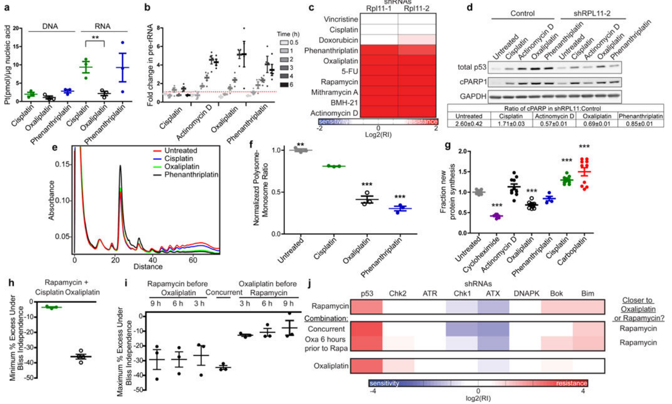
Figure 5. Oxaliplatin and phenanthriplatin induce ribosome biogenesis stress. (a) Platinum per \mu\text{g} of nucleic acid as determined by atomic absorption spectroscopy as a result of 3 h of treatment of Eu-Myc p19 Arf -/- lymphoma cells with cisplatin, oxaliplatin or phenanthriplatin at a concentration required to achieve LD80–90 at 48 h. Data are represented as mean \pm SEM from three independent doses and cultures. p < 0.005 (*) by a two-tailed Student’s t-test. (b) Percent of pre-ribosomal RNA at various time points after treatment of Eu-Myc p19 Arf -/- lymphoma cells as determined by qPCR and normalized to GAPDH. Dashed red line indicates no change. Data are represented as mean \pm SEM from four independent doses and cultures except 3 h which had five. (c) A heatmap depicting enrichment or depletion of two validated hairpins against RPL11 as a result of drug treatment in of Eu-Myc p19 Arf -/- lymphoma cells. (d) Above: western blot for total p53, cleaved PARP (cPARP) and GAPDH 12 h after treatment with or without a hairpin against RPL11 in of Eu-Myc p19 Arf -/- lymphoma cells. Below: densitometry quantification of cPARP. Shown is the ratio of cPARP in the shRPL11-2 condition relative to control for each treatment. Data are represented as mean \pm SEM from three independent densitometry quantification results. (e) Representative polysome gradient after 6 h of treatment with the indicated agents Eu-Myc p19 arf -/- cells. (f) The ratio of polysomes to monosomes normalized to the untreated condition derived from the quantification of the area under the curve of monosome and polysome fractions. Data are represented as mean \pm SEM from three technical dosing replicates. p < 0.01 (**) or p < 0.001 (***) for each group relative to cisplatin by one-way ANOVA with Dunnett’s Multiple Comparison Test. (g) Fraction of newly synthesized protein relative to the untreated
