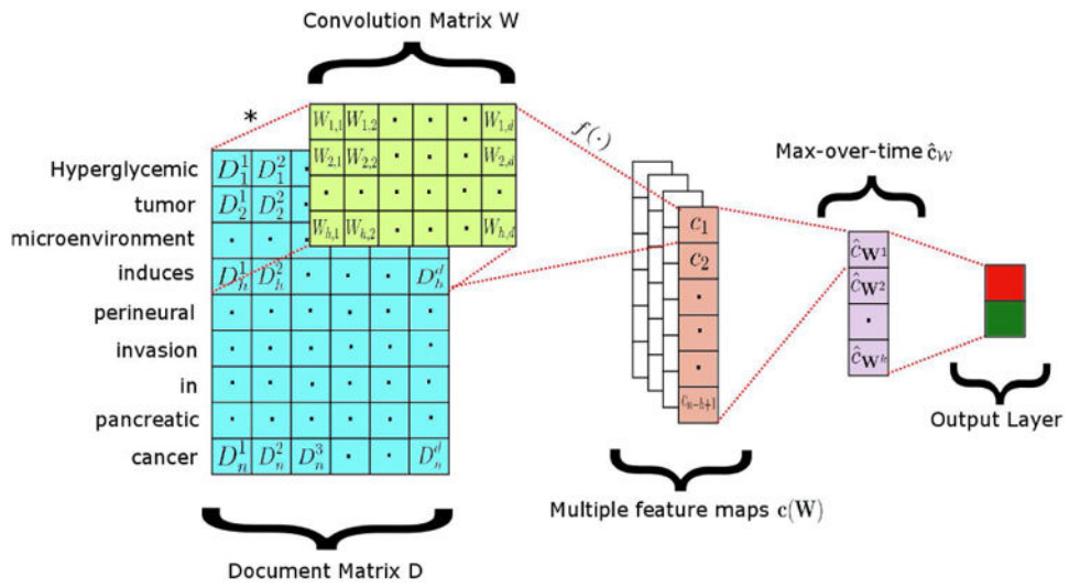
Figure 1. The CNN model layout
