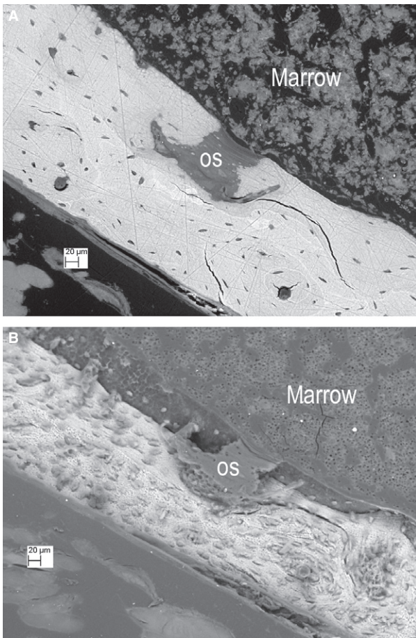
Fig. 6 Same field before and after etching. (A) Knockout (KO) tibia, PMMA-embedded ammonium triiodide stained to reveal soft tissue components, showing an osteoid patch at the centre. Surface normal to electron beam. [All other scanning electron microscopy (SEM) images in this MS were also recorded at normal electron beam incidence]. (B) The same region after 'DMG Icon-Etch' HCl gel etching for 1 min, followed by 5% NaOCl for 10 min and ammonium triiodide staining. PMMA within the osteoid patch (os) is left proud after the combined etch treatment. Osteocyte lacunae also appear as 'casts' above the etched surface. Surface tilted at 33°.
