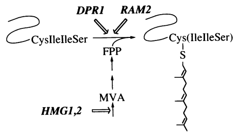
FIG. 6. Schematic representations of three yeast genes involved in farnesyltransferase. DPR1 and RAM2 genes appear to affect the farnesyltransferase directly, rather than altering the supply of farnesyl pyrophosphate (FPP) as for HMG1,2 genes. Whether they encode subunits of the enzyme has not yet been elucidated. MVA, mevalonic acid.
