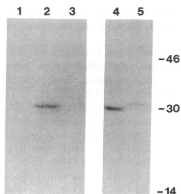
FIG. 2. SDS/polyacrylamide gel electrophoresis of the products of farnesyltransferase reaction. Farnesyltransferase reactions were carried out at 30°C with [ 3 H]farnesyl pyrophosphate (0.5 Ci/mmol). The entire sample from each reaction mixture (30 μl) was then analyzed on a 12.5% polyacrylamide gel containing SDS. Lanes: 1, UC100 extracts (50 μg) alone; 2, UC100 extracts (50 μg) + RAS2CT1 (7 μg); 3, UC100 extracts (50 μg) + RAS2CT2 (7 μg); 4, KMY2-3A extracts (121 μg) + RAS2CT1 (7 μg); 5, KMY2-3A extracts (121 μg) + f-RAS2CT1 (7 μg). Molecular mass markers indicated are ovalbumin (46 kDa), carbonic anhydrase (30 kDa), and lysozyme (14 kDa).
