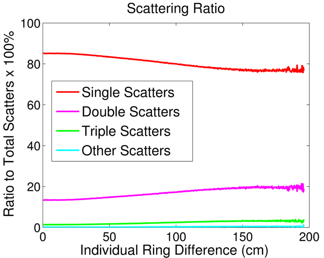
Figure 9. Fractions of single scatters and multiple scatters as a function of ring difference.
