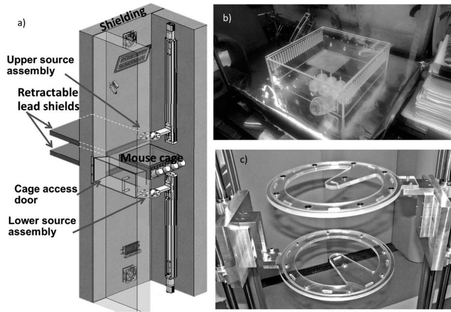
FIG. 6. Ultra-low-dose-rate irradiation system under construction.
