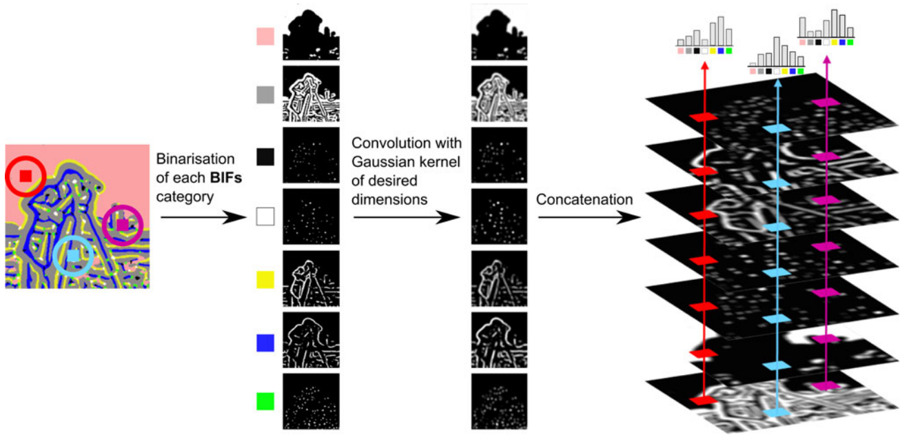
Figure 2. Construction of local soft-edged BIFs histograms. Cameraman image ©MIT.
