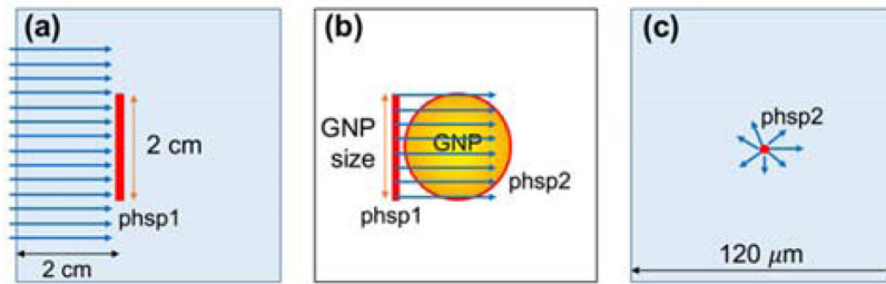
Fig. 1. Schematic diagram of simulation geometry (not in scale) (a) For 150 kVp and 51 keV photon beams, the phase space were recorded for particles passing a 2 cm diameter area at 2 cm depth in a macroscopic water phantom. (b) The radiation field was reduced to the size of GNP and irradiated into GNP in vacuum. The outgoing electrons were scored in a second phase space file on the surface of GNP. (c) The second phase space was used as source in a microscopic water phantom.
