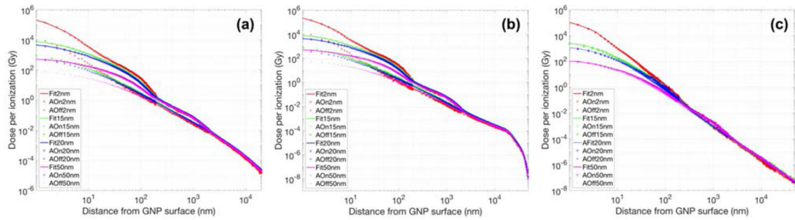
Fig. 4. Fitting curve and radial dose distributions as a function of distance from the GNP surface calculated with Monte Carlo for (a) 150 kVp, (b) 51 keV, and (c) 6 MV photon beams (AOn/AOff = with/without Auger electron contributions from atomic de-excitation processes). Results for GNP sizes of 2, 15, 20 and 50 nm are plotted.
