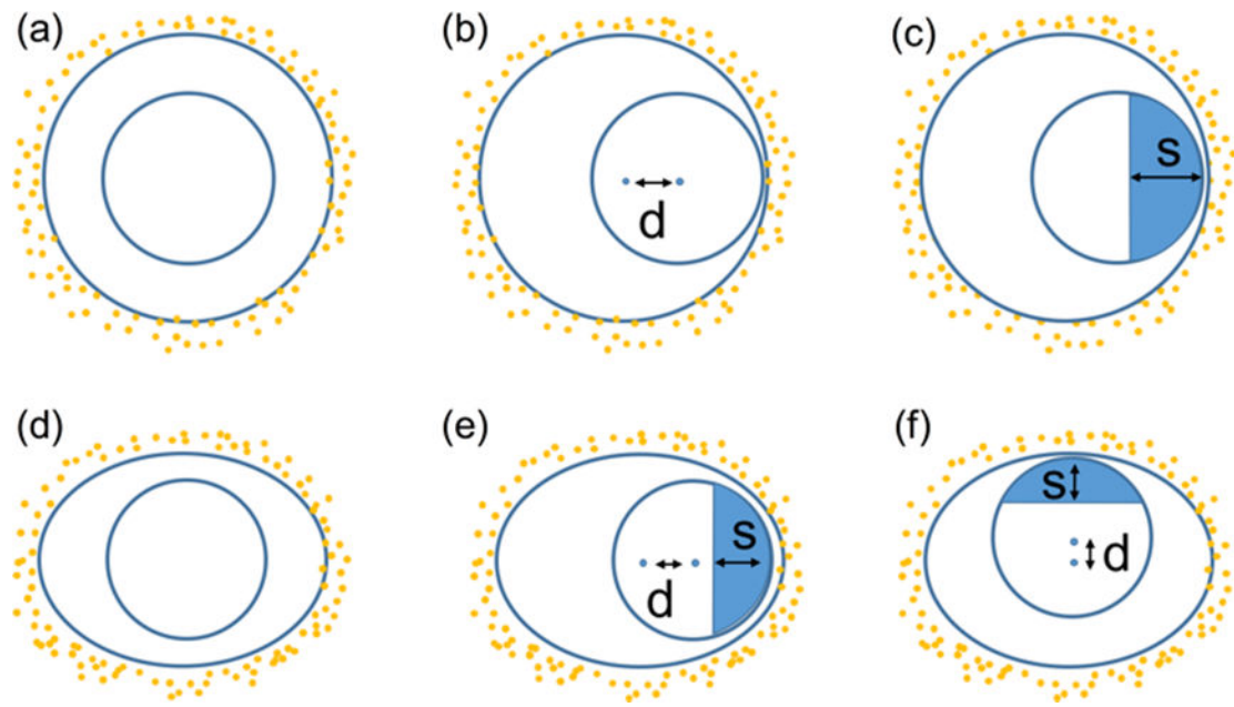
Fig. 3. Schematic diagram of cell and nucleus used for the GNP-LEM. (a): Circular cell with centrally located nucleus; (b): Circular cell with shifted nucleus; (c): Circular cell with shifted nucleus and sub-regions in the nucleus; (d)-(f): Similar for elliptical cell with nucleus shifted along major and minor axis ( d = distance between centre of cell and nucleus). The parameter s gives the size of the sub-regions in nucleus to calculate mean dose enhancement.
