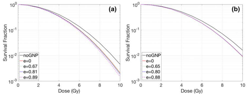
Fig. 5. Dose response curves with various eccentricities for (a) MDA-MB-231 and (b) F-98 cells. GNPs, of 15 nm diameter, were concentrated in media by a 2% weight ratio. Here e = eccentricity, a unitless quantity.
