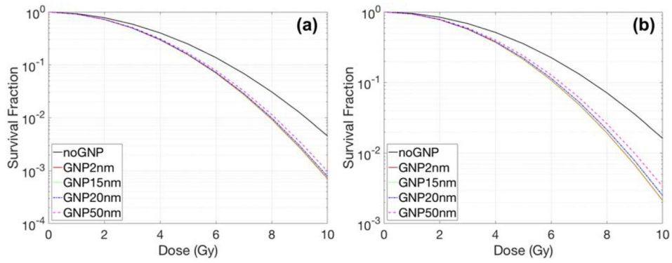
Fig. 11. Dose response curves for various GNP diameters with 150 kVp for an elliptical cell of (a) MDA-MB-231 and (b) F-98. For elliptical cells, the major/minor axis ratio is 15.5/11.5 and 44/20.5 \mu\text{m} for MDA-MB-231 and F-98 respectively. The distance between the cell and nuclear membrane was 50 nm. The GNPs were distributed in the extracellular media with a concentration of 2% by weight.
