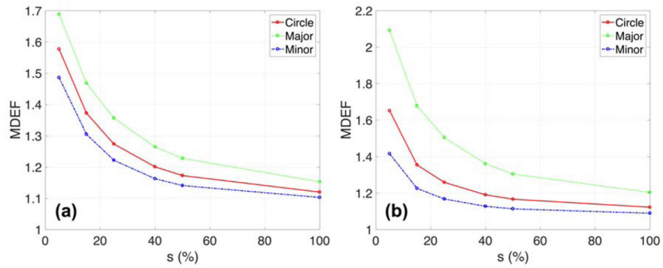
Fig. 8. Mean dose enhancement factor (MDEF) versus size of sub-regions ( s ) depending on the cell shape for (a) MDA-MB-231 and (b) F-98. For elliptical cells, major/minor cell diameters are 15.5/11.5 and 44/20.5 \mu\text{m} for MDA-MB-231 and F-98 cells. The circular nucleus was located along major/minor axis and distance between cell and nuclear membrane was 50 nm. The GNPs had a diameter of 15 nm with a concentration in the media of 2% by weight. The percentage refers to the sub-regions per nucleus diameter.
