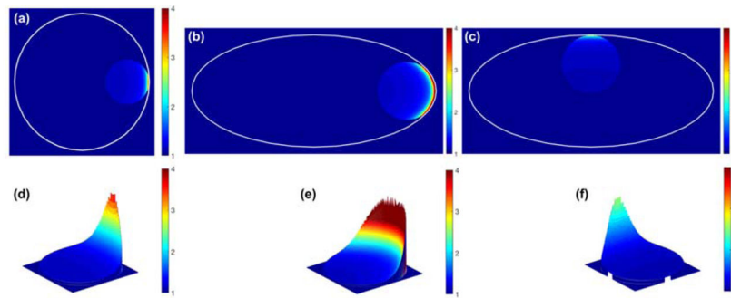
Fig. 10. Lethal event enhancement distributions for (a, d) circular and (b, c, e, f) elliptical F-98. For elliptical cells, the major/minor axis ratio is 44/20.5 \mu\text{m} for F-98 cells. The circular nucleus was located along the major/minor axis and membrane distance between cell and nucleus was 50 nm. The GNPs, of diameter 15 nm, had a concentration in the extracellular media of 2% by weight. The percentage refers to the sub-regions per nucleus diameter. The area excluding the nucleus is masked as 1.
