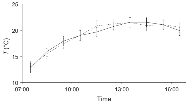
FIGURE 2 Mean hourly ambient (solid line) and internal roost (dashed line) temperatures of Barbastella barbastellus tree roosts. Temperatures were measured while bats were roosting. Error bars represent 1 standard deviation. Differences between roost and ambient temperatures are not significant (paired Student's t test, n.s.)
