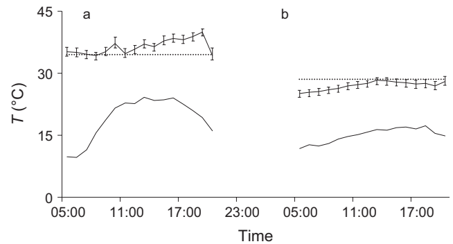
FIGURE 4 Patterns of skin temperature (solid lines with error bars) of the same female Barbastella barbastellus over two consecutive days, that is, when roosting in a group of six bats (a) and alone (b); ambient temperature (solid lines with no error bars in the lower part of the figure) and torpor onset threshold (dotted line) are also represented. Skin temperatures were not measured at night (between 21.00 and 04.00), when bats were active, but only in daytime, when they were roosting. Error bars show \pm 1 standard deviation
