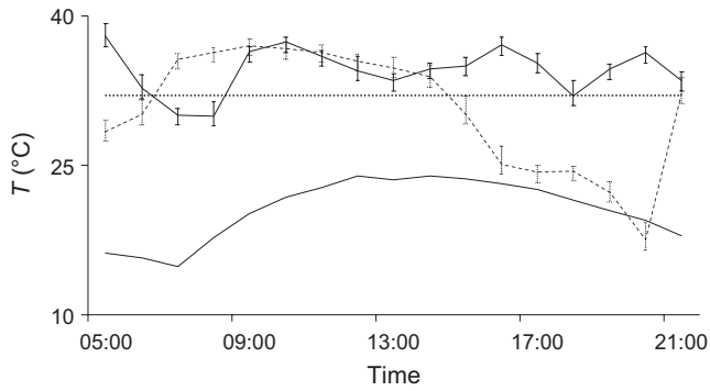
FIGURE 5 Simultaneous daily patterns of skin temperature of a male and female Barbastella barbastellus roosting in two different roosts. The upper part of the graph shows skin temperatures of male (dashed line) and female (solid line with error bars) and the torpor onset threshold (dotted line). The solid line with no error bars represents ambient temperature ( T_a ). Error bars show \pm 1 standard deviation. Times of sunrise and sunset on sampling day were, respectively, 05.48 and 20.34
