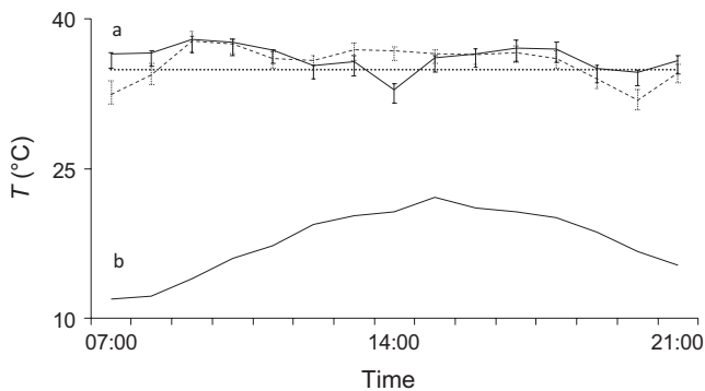
FIGURE 3 Simultaneous daily thermal patterns of two female Barbastella barbastellus roosting together in the same social group. Solid line in the upper part of the figure (a) shows skin temperature of a nonreproductive female, dashed line that of a lactating female; point line: torpor onset threshold. Solid line in the lower part of the figure (b) shows ambient temperature. Error bars show \pm 1 standard deviation. Sunrise and sunset times on sampling day were, respectively, 05.45 and 20.36
