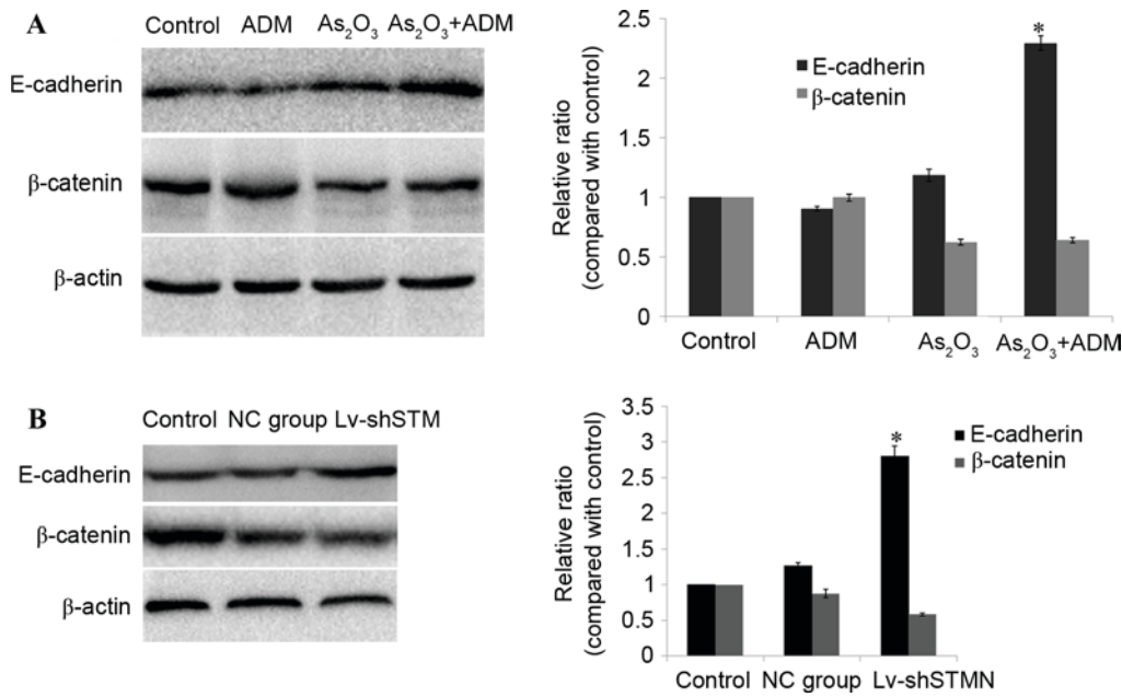
Figure 5. Effect of As 2 O 3 and ADM combination treatment on E-cadherin and β-catenin expression levels. (A) The cells were treated with 2 μM As 2 O 3 and/or 200 ng/ml ADM for 48 h. A western blot analysis was used to quantify the expression of E-cadherin and β-catenin. (B) Lv-shSTMN and NC were transfected into the cells. A western blot analysis was used to detect the expression of E-cadherin and β-catenin. The immunoreactive bands of E-cadherin and β-catenin protein were normalized to β-actin. *P<0.05 compared with control group. As 2 O 3 , arsenic trioxide; ADM, doxorubicin; Lv-shSTMN, lentivirus with small hairpin RNA against stathmin; NC, negative control virus.
