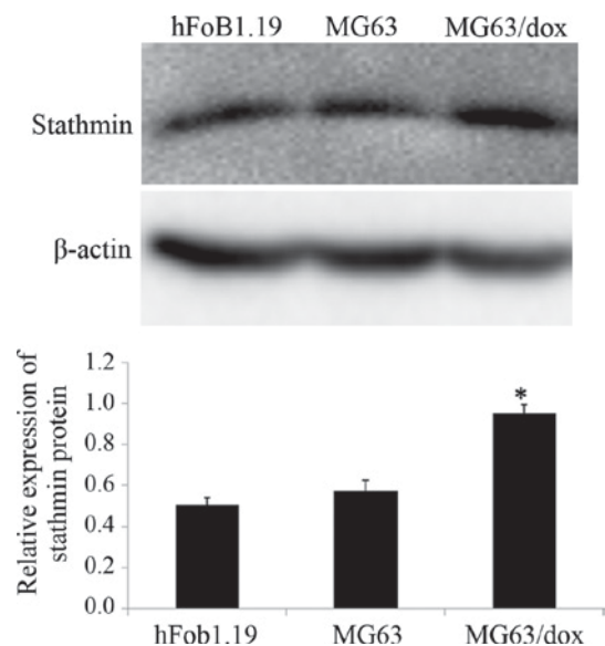
Figure 1. Quantification of the expression level of stathmin in human osteosarcoma cells (MG63 and MG63/dox) and osteoblast cells (hFoB1.19), compared with \beta -actin. Western blotting was employed to detect the expression of stathmin protein. The data are expressed as the mean \pm standard deviation. *P<0.05 compared with hFoB1.19. MG63/dox, MG63/doxorubicin-resistant.
