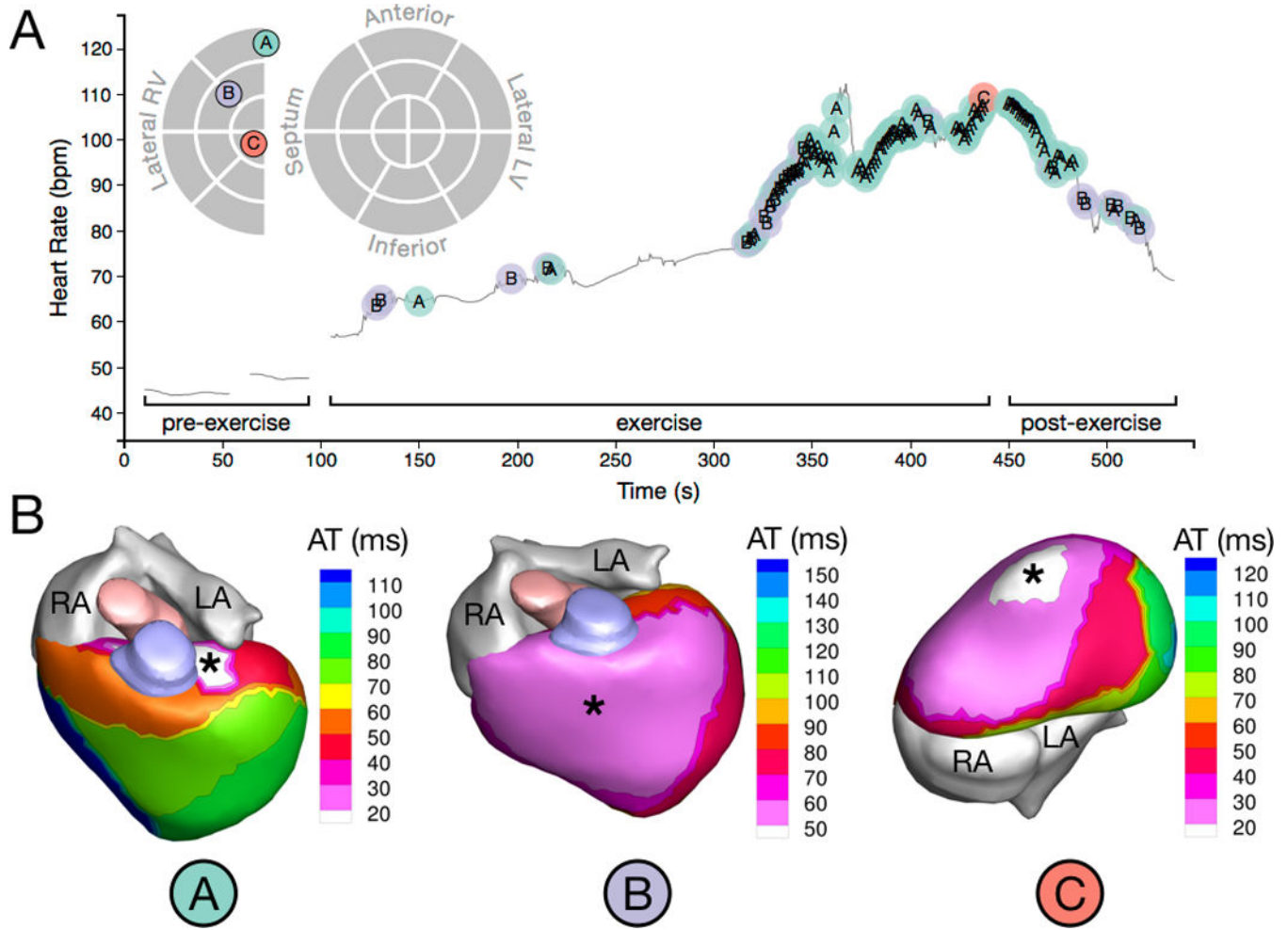
Figure 6. PVC onset and initiation sites of a patient (Patient 6) with a high PVC burden (18.69%). (A) Time-course of observed PVCs in relation to exercise and schematic map of PVC initiation sites. The different PVC initiation sites are labeled A, B, and C and color coded. PVCs occurred only after the onset of exercise, and morphology C appeared only once near peak HR (B) Activation isochrone maps of the three distinct PVC morphologies observed in this patient. Asterisks indicate PVC initiation sites. Morphology B showed very a broad region of early epicardial activation, indicating a possible sub-epicardial origin and possible conduction system involvement. HR: heart rate.
