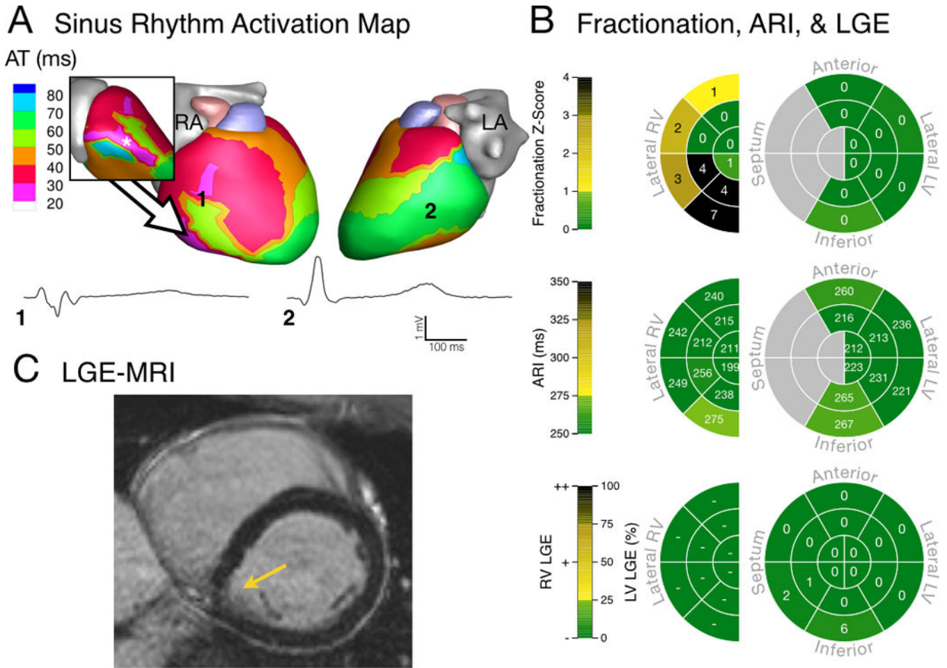
Figure 4. Electrical substrate of a 26-year-old male (Patient 13) with early disease and no observed PVCs. (A) Sinus rhythm epicardial breakthrough occurred in the inferolateral RV (asterisk in inset) with early activation of the RV free wall. There was a region of non-uniform conduction and fractionated unipolar EGMs (1) between these sites. Remote LV unipolar EGM (2) had a normal morphology. (B) Fractionation in the RV was much greater than control values (top) while Fridericia-corrected ARI values were within the normal range of controls (middle). Minimal LGE was visible in the LV (bottom). (C) MRI showed minimal abnormalities (arrow).
