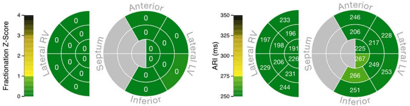
Figure 1. Electrical substrate in a healthy adult. (A) Sinus rhythm activation with a typical RV epicardial breakthrough (asterisk) and normal conduction. RV (1) and LV (2) unipolar EGMs have a normal morphology free of fractionation. (B) Schematic maps of normal electrical properties in anatomical regions based on 20 control subjects. Left: fractionation z-score. Right: Fridericia-corrected ARI. The maps show absence of fractionation and ARI values within the normal range. AT: activation time. RA: right atrium. LA: left atrium. RV: right ventricle. LV: left ventricle. ARI: activation-recovery interval. EGM: electrogram.
