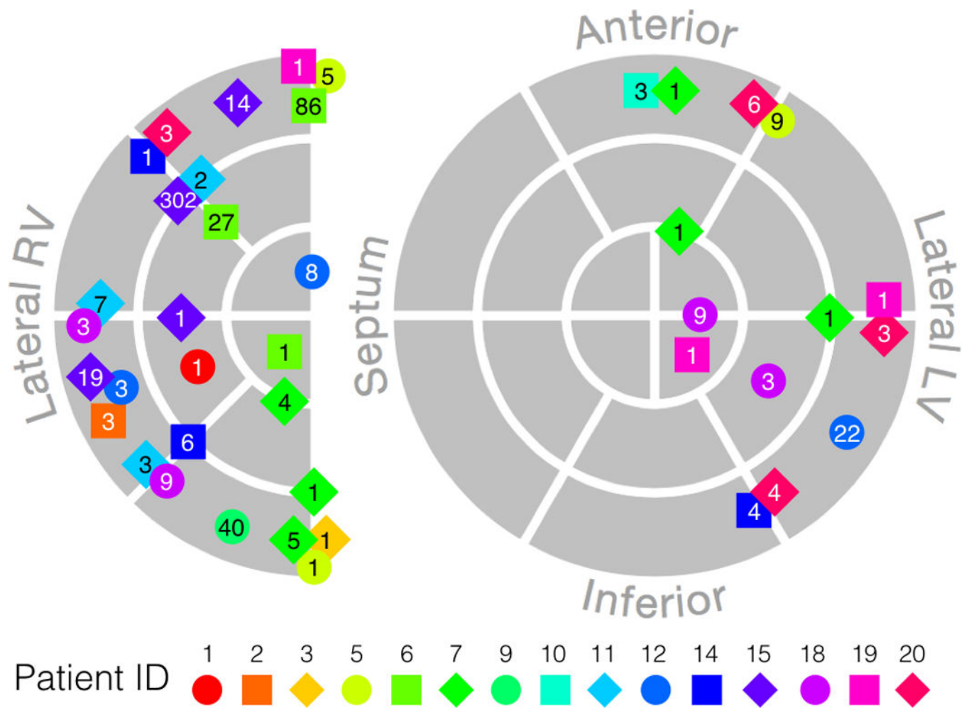
Figure 5. Schematic diagram of earliest epicardial activation of all observed PVC morphologies. Each marker represents a unique PVC morphology, with the number indicating the number of times the morphology was observed during the study. Marker color and shape identify patient ID (indicated below diagram). Sites near the epicardial aspect of the septum are shown on the edge of the RV.
