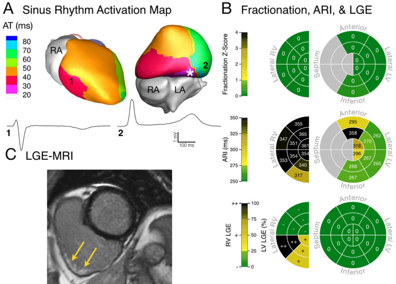
Figure 2. Electrical substrate of a patient (Patient 6) with advanced disease and a high PVC rate (18.69%). (A) Ventricular epicardial breakthrough during sinus rhythm was abnormal, with earliest activation originating from the basal inferior LV (asterisk). RV (1) and LV (2) unipolar EGMs had normal QRS morphology. (B) EGM fractionation was not abnormal compared to controls (top). Fridericia-corrected ARIs were prolonged compared to control values (middle). Concentrated LGE was visible in the inferior RV (bottom). (C) MRI image of extensive LGE, which was confined to the subepicardial RV (indicated by yellow arrows). PVC: premature ventricular contraction.
