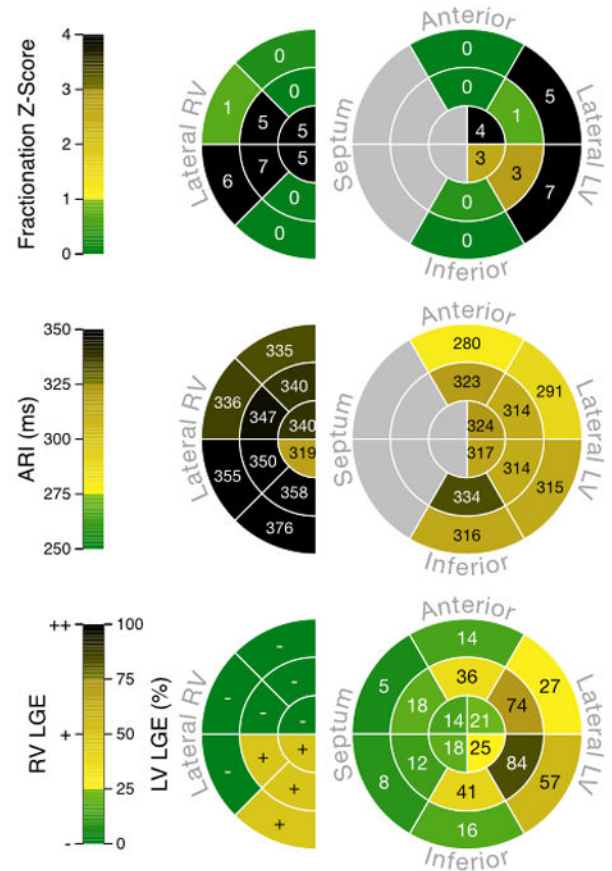
Figure 3. Electrical substrate of a patient (Patient 14) with biventricular disease and a moderate PVC rate (1.11%). (A) Sinus rhythm breakthrough was abnormal, with earliest epicardial activation originating from the basal lateral LV (asterisk). RV (1) and LV (2) unipolar EGMs were fractionated (note the voltage scale of low-amplitude EGM 1). (B) Regions of high fractionation were present in both ventricles (top), and Fridericia-corrected ARI values were prolonged compared to control values (middle). LGE was visible in both ventricles (bottom). (C) MRI image of LGE showing scar in both ventricles (yellow arrows).
