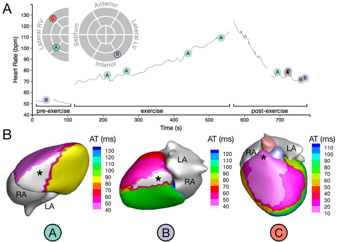
Figure 7. PVC onset and initiation sites of a patient (Patient 14) with a moderate PVC burden (1.11%). (A) Time-course of observed PVCs in relation to exercise and schematic map of PVC initiation sites. Note that morphology C is partially obscured in the post-exercise recording period. (B) Activation isochrone maps of the three distinct PVC morphologies observed in this patient. Asterisks indicate PVC initiation sites.
