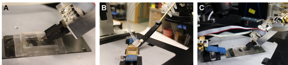
FIG. 7. Interface schemes for the functionalized SU-8 microfluidic probe. (a) A PCB is connected to the probe tip (to interface the active and reference electrodes); (b) another PCB is connected to the substrate by a spring contact (to interface the counter electrode). The signals are transferred to the impedance analyzer (black box) that is connected to the computer. The fluidic connection between the pipette channels and the liquid reservoirs is arranged with a PDMS fluid-coupling piece in which the tubes are inserted. (c) Side-view of the interface.
