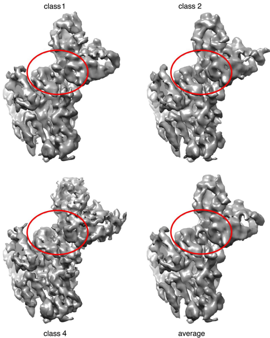
Fig. 5. Density from classes 1,2, and 4 for an HA "head" and bound scFv and average of the three superposed on the region shown in the red ovals. There was a slight enhancement of density at the interface, helpful for building the CDRH3 loop.
