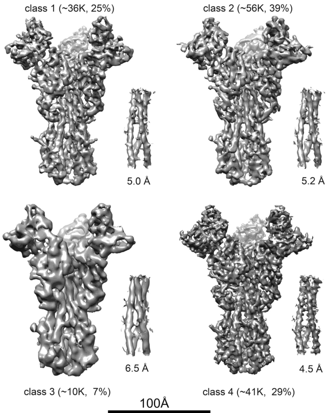
Fig. 3. Surface representations of 3D class averages for HA:scFv complex. The labels include the number of particles in each class and the corresponding percentage of the total particles included in the computation. Beside each map is a detail from the long central helix of HA 2 , to illustrate resolution differences among the classes. The resolutions given are from the half-map FSC for each class (see Fig. S4, which also includes the FSC for each map with its corresponding refined model).
