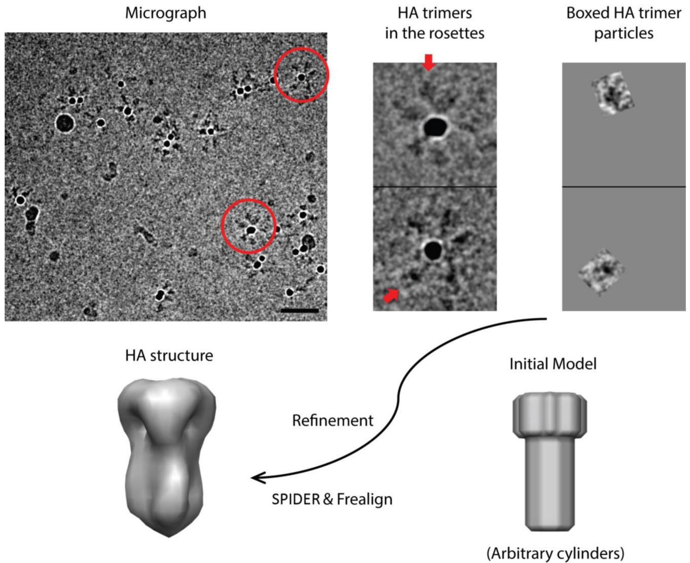
Fig. 1. Use of gold-bead HA rosettes to derive starting model. Upper row: (left) a field from a cryomicrograph with two rosettes in red circles, scale bar = 500 Å; (center) magnified images of those two rosettes, with arrows indicating the HA trimers shown boxed on the right. An arbitrary, cylindrical model (one example shown) led to the low-resolution HA trimer model, used for subsequent work.
