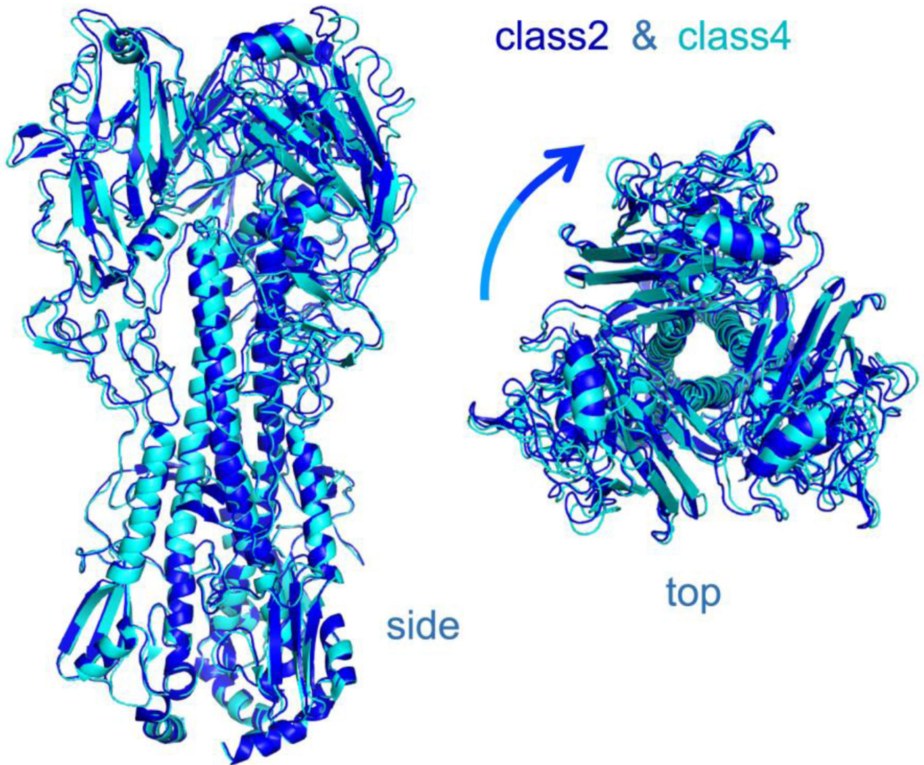
Fig. 4. Superposition of class 2 (blue) and class 4 (cyan) models, illustrating difference in twist around the threefold axis. The models were fit to the final reconstructions by real-space refinement and inspection shows that they accurately represent the key differences between the two maps. The two models are aligned at the base of HA 2 , so that a relative circumferential displacement of the upper surface of HA 1 illustrates the overall twist of the molecule. Both views include only the HA part of the model. The top view (right) shows about a 10° rotation of one head with respect to the other.
