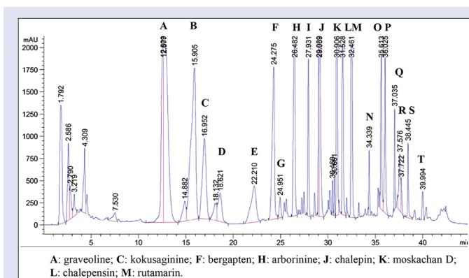
Figure 1: High-performance liquid chromatography chromatogram of the chloroform extract of Ruta angustifolia Pers. The chloroform extract of Ruta angustifolia Pers. was subjected to high performance liquid chromatography analysis, and twenty fractions corresponding to peaks A–T were collected and identified
