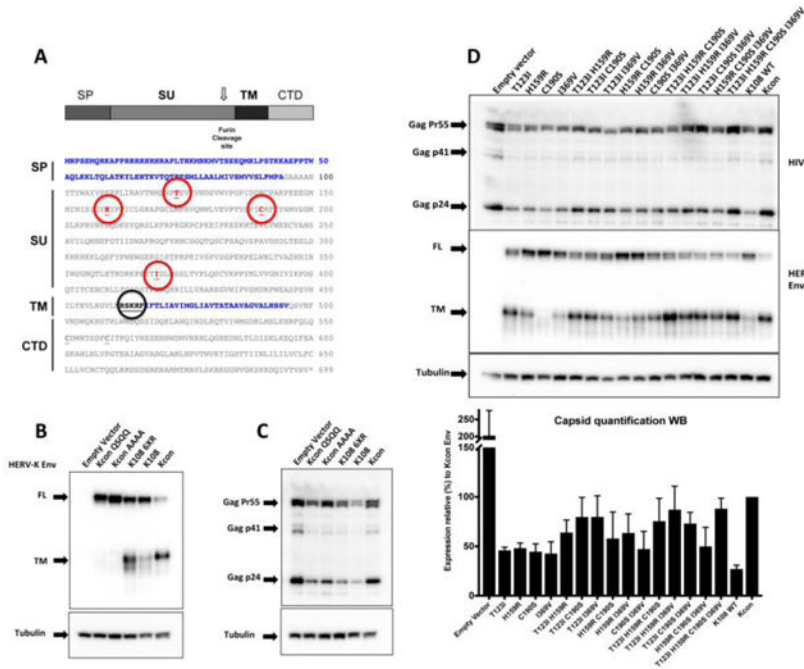
Figure 4. A) Schematic representation of HERV-K con and HERV-K108 envelope sequences. The positions where the residues differ between HERV-K108 and HERV-Kcon are identified by red circles. The black circle highlights the furin cleavage site. SP stands for signal peptide (shown as a blue sequence), SU stands for surface domain, TM for transmembrane (TM ectodomain shown blue sequence) and CTD stands for cytoplasmic domain. B) and C) Effect of furin cleavage site mutagenesis on the interference on HIV by HERV-K108 Env. Disruption of furin cleavage site inhibits HERV-Kcon Env processing and increases its inhibitory effect on HIV production, while optimization of the furin cleavage site increases HERV-K108 Env processing but does not rescue HIV-1 production. FL stands for full-length and TM for transmembrane domain. D) Mutagenesis of all four residues that differ between K108 and Kcon rescues HIV-1 production. Western blot of lysates of HEK 293T co-transfected with 250ng of HIV-1 pLAI2, 100ng pcRV1-K rev and 60ng of HERV-K108 env versions harboring all possible combinations of the 4 mutant residues as well as HERV-Kcon env . Quantifications reflect the average of three independent experiments and the error bars represent the standard deviation from the mean. FL stands for full-length and TM for transmembrane domain.
