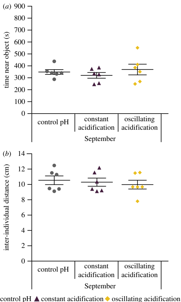
Figure 3. Immediately after the shoaling test, a novel object was placed into the arena and shoal behaviour was recorded for 900 s ( n = 6 shoals per treatment). (a) Time near novel object was not affected by CO 2 /pH treatments ( F_{2,15} = 0.159, p = 0.855 ). (b) Inter-individual distance to conspecifics was also not affected by CO 2 /pH treatments ( F_{2,15} = 0.312, p = 0.737 ). Data presented as mean \pm s.e.m. This test was only performed on the September groups.
