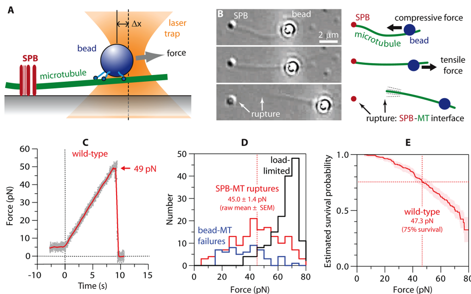
FIGURE 2: Measuring the strength of individual SPB–microtubule attachments. (A) Beads decorated with kinesins (in the absence of ATP, i.e., in “rigor”) form strong linkages to the microtubules, allowing application of high forces to individual SPB–microtubule attachments using a laser trap. (B) The laser trap (not visible) applies force to a bead linked to an SPB-attached microtubule (MT). Top, initially, the trap pushes the bead toward the SPB, applying compressive force to the SPB-MT interface and causing the MT to buckle. Middle, the direction of force is reversed to apply tensile force to the SPB-MT attachment. Bottom, after the SPB-MT interface ruptures (arrows), the filament remains linked to and pivots around the trapped bead. The SPB appears slightly different in this image due to a slight change in microscope focus. See also Supplemental Movie S2. (C) Tensile force vs. time (force ramp, 5 pN/s) applied to a microtubule attached to a wild-type SPB. Grey dots show raw data. Red trace shows the same data after smoothing (500-ms sliding boxcar average). Dashed vertical line marks the start of the force ramp. Arrow marks rupture at the SPB–microtubule (SPB-MT) interface. (D) Histograms showing outcomes from a series of force ramp experiments using wild-type SPBs. Vertical dashed line marks raw the mean rupture force, computed from only the subset of trials ending with SPB–microtubule rupture. (E) Survival probability as a function of force for microtubule attachments to wild-type SPBs, estimated using Kaplan–Meier analysis. Shaded area shows 95% confidence intervals. Dashed vertical line marks the estimated force at 75% survival.
