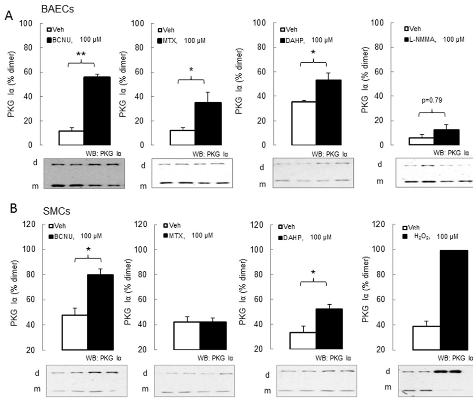
Fig. 1. In vitro treatment of cells with NOS-uncoupling drugs results in robust PKG Iα disulfide dimerization. (A) Bovine aortic endothelial cells (BAECs) treatment with BCNU, MTX or DAHP (100 μM for 3 h) resulted in significant increase of PKG Iα disulfide dimerization, whereas treatment with L-NMMA (100 μM for 3 h) did not. (B) Smooth muscle cells (SMCs) treatment with BCNU or DAHP (100 μM for 6 h) resulted in significant increase of PKG Iα disulfide dimerization, whereas treatment with MTX (100 μM for 6 h) did not. A positive control, namely 100 μM H 2 O 2 for 30 min, causes nearly all PKG Iα to disulfide dimerize. n = 6–8/group. Data represented as mean ± SEM. *P ≤ 0.05, **P ≤ 0.01 versus vehicle treatment.
