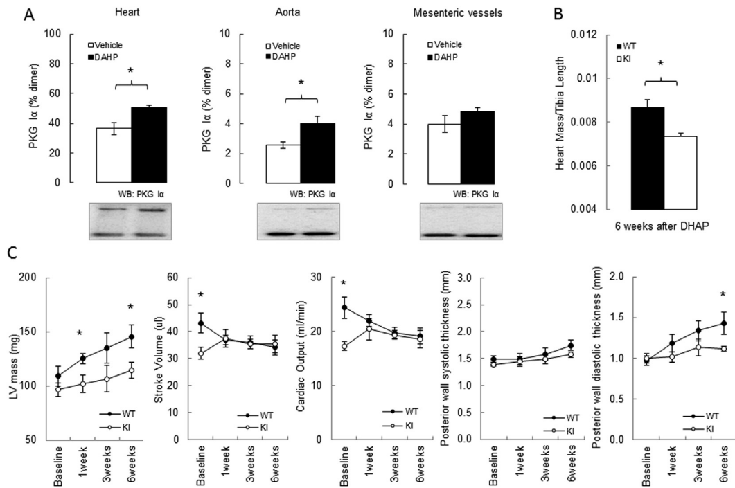
Fig. 2. In vivo treatment with DAHP causes PKG Iα disulfide dimerization and adaptive cardiac structural and functional abnormalities. (A) Increase of PKG Iα disulfide dimerization in heart or aorta, but not in mesenteric vessels from mice treated with DAHP (10 mM in the drinking water for 3 weeks). (B) Heart mass to tibia length ratio was lower in the KI mice compared to WT after 6 weeks of treatment with DAHP. (C) Time-dependent changes in left ventricular (LV) mass, stroke volume, cardiac output and posterior wall thickness at the baseline and during 1, 3 and 6 weeks of DAHP treatment in WT and KI mice. n = 6/group. Data represented as mean ± SEM. *P ≤ 0.05, versus vehicle treatment (A) or versus KI (B and C).
