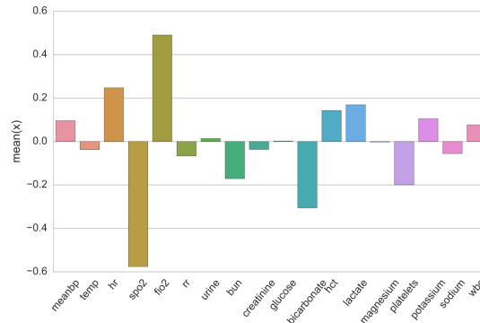
Figure 4: Average value of dynamic features x_{nt} assigned to timesteps strongly associated with state index 9. Values are z-score standardized per variable. State 9 had very low observed spo2 and bicarbonate levels as compared to other states. Lactate levels were the highest observed across all states - no other state had significant positive lactate z-scores.
