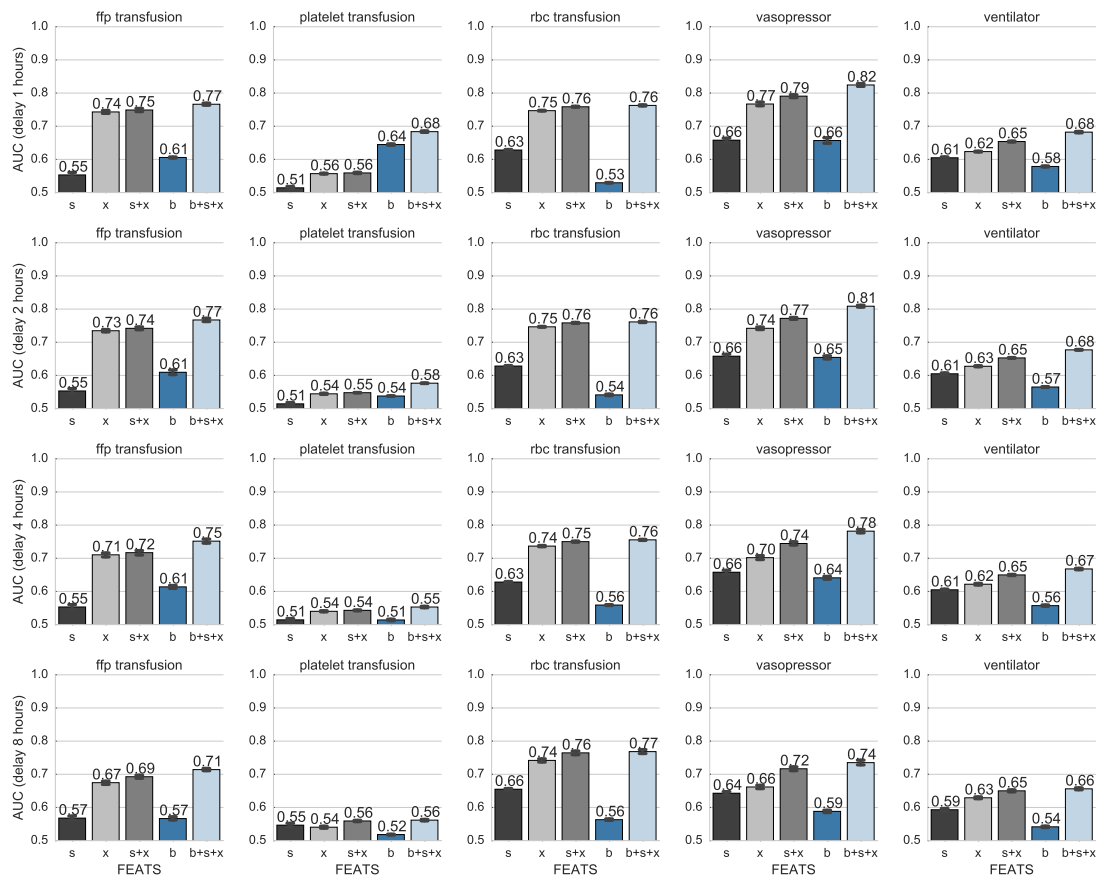
Figure 2: AUC scores for different features predicting the onset of each intervention at a delay of d \in \{1, 2, 4, 8\} hours ahead of the current timestep. Features : Each bar color denotes one feature or feature concatenation: static observations s (10 dimensions using one-hot encoding), dynamic time-series observations x (18 dimensions), and belief state vectors b ( K = 10 dimensions) from the switching state model in Eq. (2). Interventions : fresh-frozen-plasma transfusion (ffp), platelet transfusion, red-blood-cell (rbc) transfusion, vasopressor administration, and ventilator intubation.
