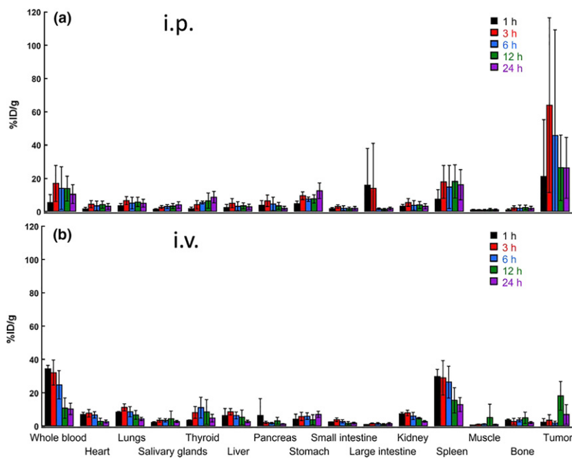
Fig. 2. Biodistribution of astatine-211-labeled trastuzumab ( ^{211}\text{At} -trastuzumab) in a mouse model of peritoneal metastasis of gastric cancer. Uptakes (percent injected dose per gram of tissue [%ID/g]) of ^{211}\text{At} in the tumor and other organs at 1, 3, 6, 12, and 24 h after i.p. (a) or i.v. (b) injection of ^{211}\text{At} -trastuzumab (1 MBq). Five (for i.p. injection) or four (for i.v. injection) mice were used at each time point. All data represent mean \pm SD.
