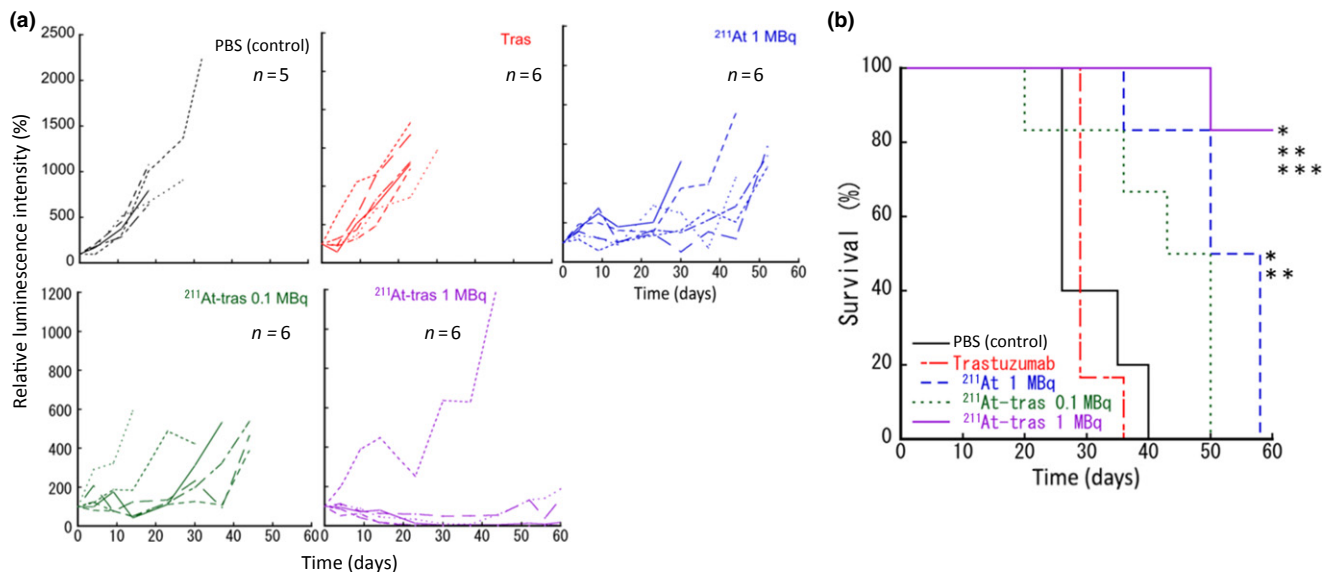
Fig. 4. Therapeutic results of locoregional therapy with astatine-211-labeled trastuzumab ( ^{211}\text{At} -tras) in the xenograft mouse model of peritoneal metastasis of gastric cancer. (a) Quantified relative tumor luminescence intensities in each mouse enrolled in this study. The luminescence intensity before the treatment was considered to be 100%. Six mice were enrolled in each of the treatment groups, except the control (five mice). (b) Kaplan–Meier survival curves of mice. * P < 0.05 versus control; ** P < 0.05 versus Tras; *** P < 0.05 versus ^{211}\text{At} .
