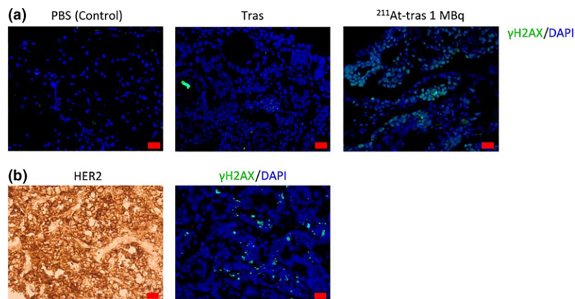
Fig. 7. \gamma H2AX foci in a mouse model of peritoneal metastasis of gastric cancer (PMGC). (a) \gamma H2AX foci in PMGC cells at 6 h post-injection with PBS, unlabeled trastuzumab (Tras), or 1 MBq of astatine-211-labeled trastuzumab ( ^{211}\text{At} -tras). Scale bar = 20 \mu\text{m} . (b) Human epidermal growth factor receptor 2 (HER2) and \gamma H2AX foci in PMGC cells at 3 h post-injection with 1 MBq ^{211}\text{At} -tras. Scale bar = 20 \mu\text{m} .
