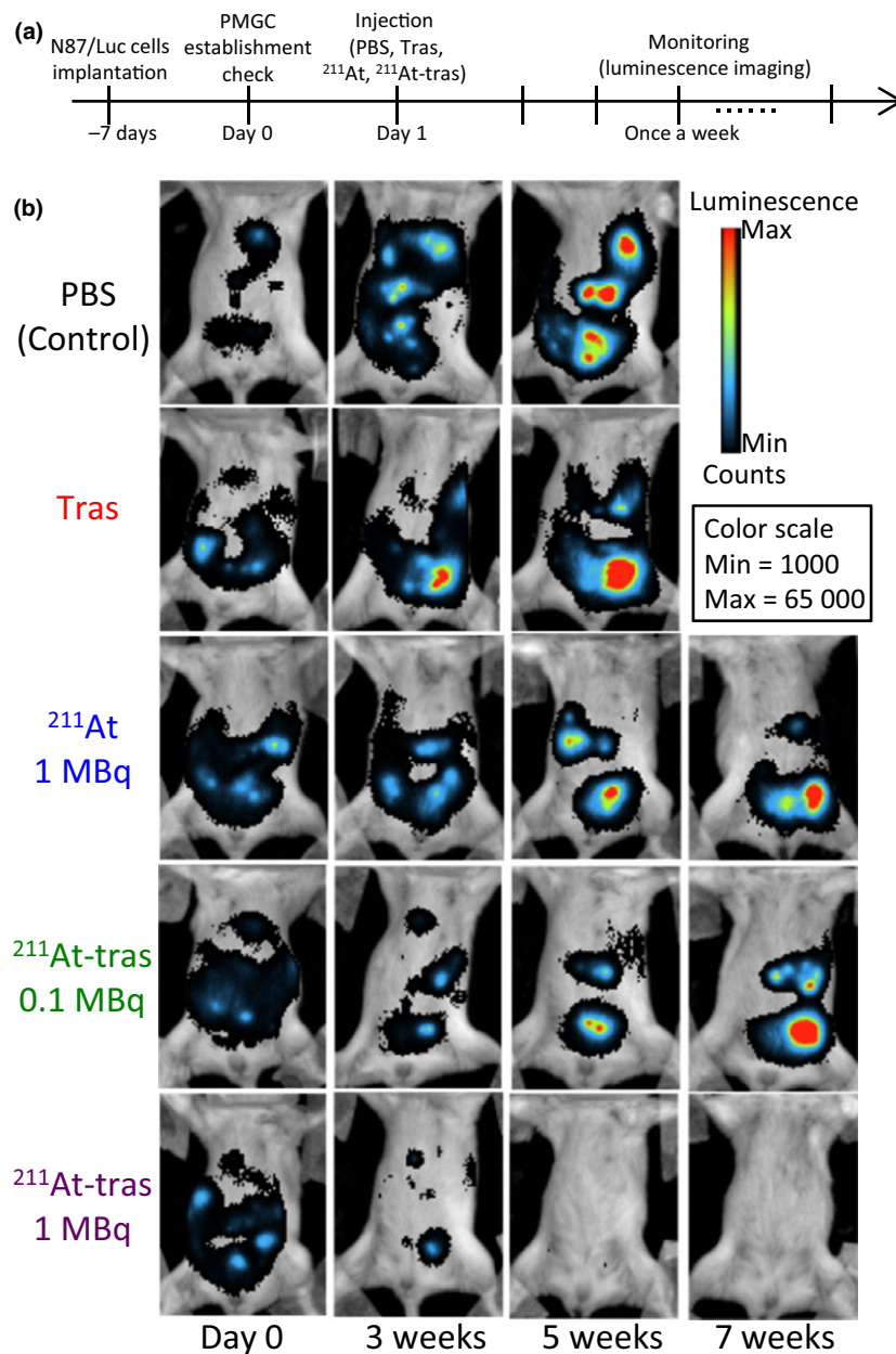
Fig. 3. Locoregional therapy with astatine-211-labeled trastuzumab ( ^{211}\text{At} -tras) in a mouse model of peritoneal metastasis of gastric cancer (PMGC), and tumor monitoring. (a) Treatment schedule. (b) Representative bioluminescence images of tumor growth in the mouse model treated with PBS (control), unlabeled trastuzumab (Tras), ^{211}\text{At} (1 MBq), or ^{211}\text{At} -tras (0.1 or 1 MBq). Images were captured on the day before treatment (Day 0) or at 3, 5, or 7 weeks (w) after treatment. The color scale indicates the luminescence intensity per pixel.
