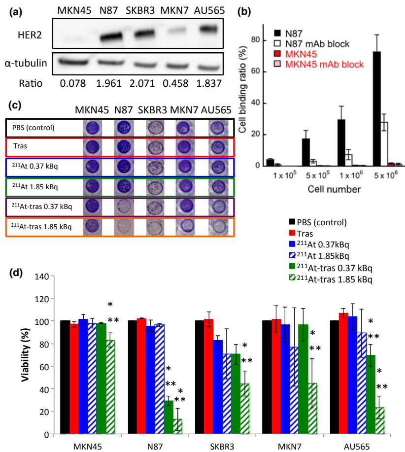
Fig. 1. In vitro analysis of cell binding by astatine-211-labeled trastuzumab ( ^{211}\text{At} -tras) and subsequent cell death. (a) Human epidermal growth factor receptor 2 (HER2) expression in MKN45, N87, SKBR3, MKN7, and AU565 cells. \alpha -Tubulin was used as a loading control. Ratios of the band intensity of HER2 relative to \alpha -tubulin are indicated below the images. (b) Cell binding ratio of ^{211}\text{At} -trastuzumab to N87 and MKN45 cells with/without trastuzumab (mAb) block. Bars are labeled in the graph. Three independent experiments were carried out, each in triplicate ( n = 3 ). (c) Representative images of stained surviving cells at 7 days after 24 h of treatment with PBS control, unlabeled trastuzumab (Tras), ^{211}\text{At} (0.37 or 1.85 kBq), or ^{211}\text{At} -tras (0.37 or 1.85 kBq). (d) Quantification of the viability of the cells in panel (c) treated with ^{211}\text{At} -tras for 7 days. Bars are labeled in the graph. Three independent experiments were carried out in triplicate ( n = 3 ). All data represent mean \pm SD. * P < 0.05 versus control; ** P < 0.05 versus Tras.
