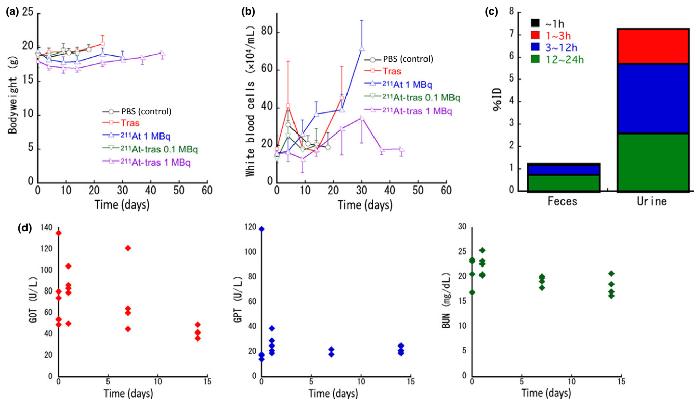
Fig. 5. Side-effects and excretion of astatine-211 ( ^{211}\text{At} ) in a mouse model of peritoneal metastasis of gastric cancer treated with ^{211}\text{At} -labeled trastuzumab ( ^{211}\text{At} -tras). (a) Bodyweight of the mice after treatment. Plots were interrupted if the animal reached the defined endpoint. Data represent mean \pm SD. (b) White blood cell counts in the mice after treatment. Plots were interrupted if the animal reached the defined endpoint. Data represent mean \pm SD. (c) ^{211}\text{At} levels in feces and urine of the mice up to 24 h after i.p. injection of ^{211}\text{At} -tras (1 MBq). Six mice were used in the experiment. The bars represent the cumulative mean values obtained over a 24-h observation period. Bars are labeled in the graph. (d) Glutamic oxaloacetic transaminase (GOT; red), glutamic pyruvate transaminase (GPT; blue), and blood urea nitrogen (BUN; green) values up to 14 days after i.p. injection of ^{211}\text{At} -tras (1 MBq). Five mice were used for 0 and 1 days, and four mice were used for 7 and 14 days. Data for each mouse are shown in the graph.
