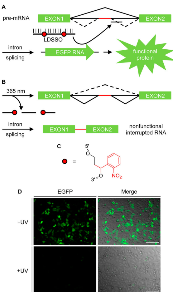
Figure 2. Optochemical regulation of splice switching with the LDSSO for an ON → OFF gene expression light switch. Schematics for the two RNA splicing pathways (black) and the mutant intron (red) are shown. (A) In the absence of irradiation, the LDSSO binds to the target site for aberrant splice correction and activation of gene expression. (B) UV cleavage of the LDSSO deactivates splice correction, and gene expression is interrupted by the mutant intron. (C) Red circles represent ONB linker residues, with the photo-cleavable group indicated in red. (D) HeLa:EGFP654 cells were transfected with the LDSSO, irradiated for 2 min or kept in the dark, and imaged for EGFP expression after 24 h. Images of the EGFP channel (left) and the EGFP channel merged with a brightfield image (right) are shown. Scale bars indicate 0.2 mm.
