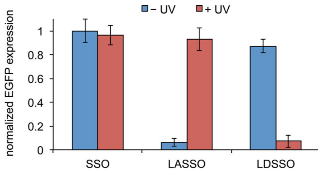
Figure 3. Flow cytometry quantification of optically regulated splice-switching with LASSO and LDSSO. HeLa:EGFP654 cells were transfected with the SSOs, irradiated for 2 min or kept in the dark, and analyzed for EGFP expression after 24 h. The gated EGFP positive cells were normalized to the noncaged control. Error bars represent standard deviations from three independent experiments through counts of 20 000 cells each.
