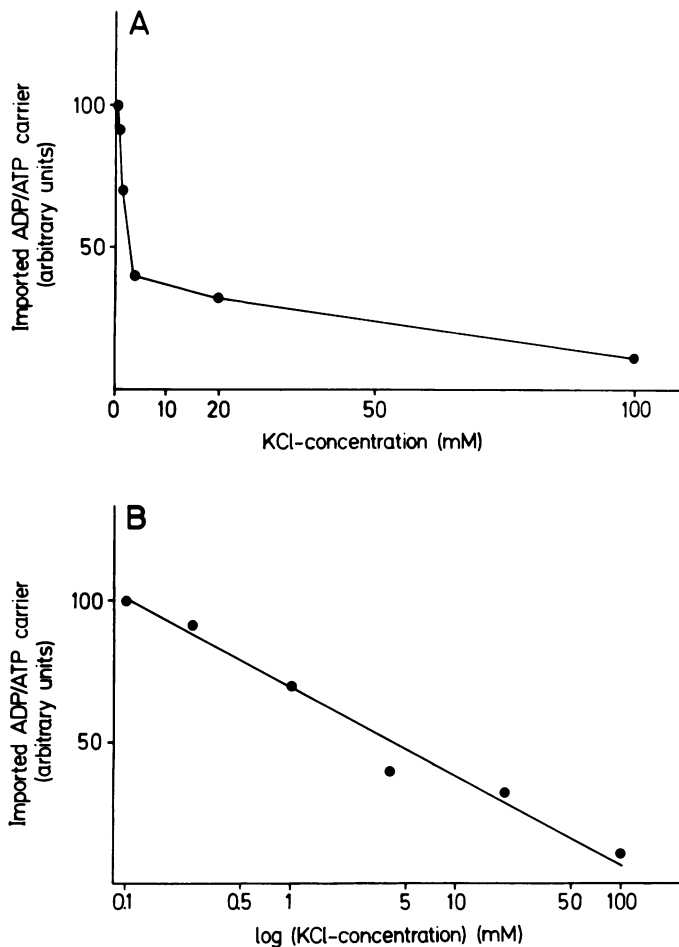
Fig. 4. Import driven by a potassium diffusion potential. Samples containing 35 \mu\text{l} ^{35}\text{S} -labelled reticulocyte lysate, isolated mitochondria ( 25 \mu\text{g} protein), 0.1 \mu\text{M} valinomycin, 4 \mu\text{M} antimycin A and 10 \mu\text{M} oligomycin, were incubated for 25 min at 25^\circ\text{C} . After cooling to 0^\circ\text{C} , mitochondria were re-isolated and re-suspended in 300 \mu\text{l} buffer (pre-warmed to 25^\circ\text{C} ) containing valinomycin, antimycin A and oligomycin at the same concentrations as mentioned above. The buffer was 0.25 \text{ M} sucrose, KCl and NaCl at a total concentration of 100 \text{ mM} , 5 \text{ mM} \text{MgCl}_2 , 3\% (w/v) BSA and 10 \text{ mM} MOPS, adjusted to pH 7.2 with NaOH; KCl concentrations were 0.1, 0.25, 1, 4, 20 and 100 \text{ mM} , respectively. After 3 min at 25^\circ\text{C} and 15 min at 0^\circ\text{C} samples were assessed for protease-resistant ADP/ATP carrier associated with mitochondria. The KCl concentrations at the final 25^\circ\text{C} incubation are plotted on a linear scale in (A) and on a logarithmic scale in (B).
