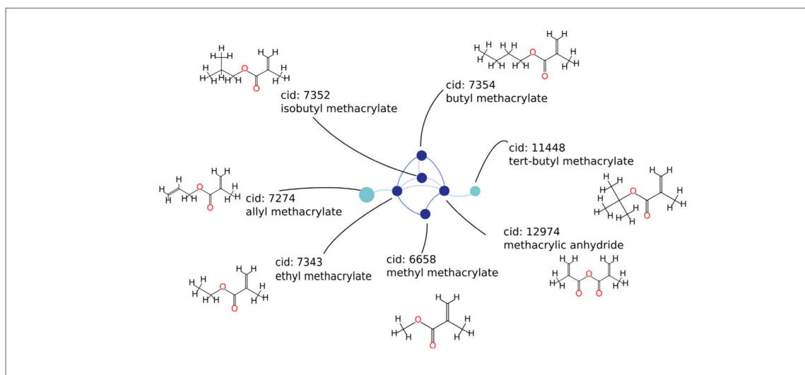
Fig. 7. Module 1 similarity subgraph with methacrylate Michael's acceptors of Figure 6 Edges drawn for substructure similarity > 90%. Dark blue signifies a skin sensitizer, light blue a non-sensitizer.
