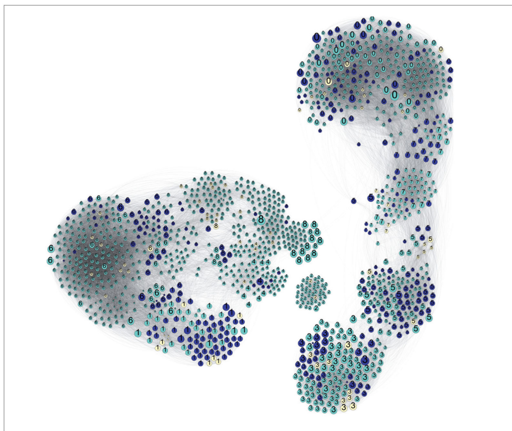
Fig. 6. Chemical similarity network with experimentally classified sensitizers from REACH (registered 2008–2014) mapped to PubChem
