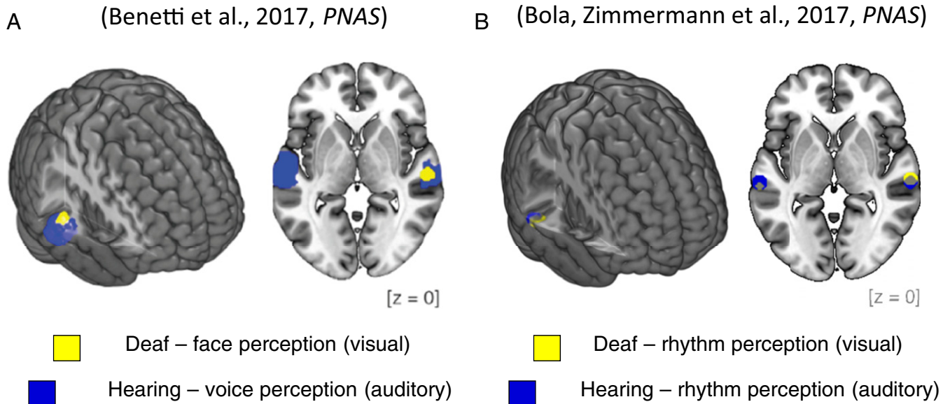
Fig. 1. Task-specific auditory cortex reorganization in deaf humans. Cross-modal plasticity in the auditory cortex of congenitally deaf people overcomes the division between visual and auditory processing streams, as regions of high-level auditory cortex become recruited for visual face processing and visual rhythm perception. (A) fMRI results show peaks of activation for auditory voice recognition in the hearing (blue) and for visual face recognition in the deaf (yellow). Reproduced from ref. 2. (B) fMRI results also show peaks of activation for auditory rhythm perception in the hearing (blue) and visual rhythm perception in the deaf (yellow). Adapted from ref. 13.
